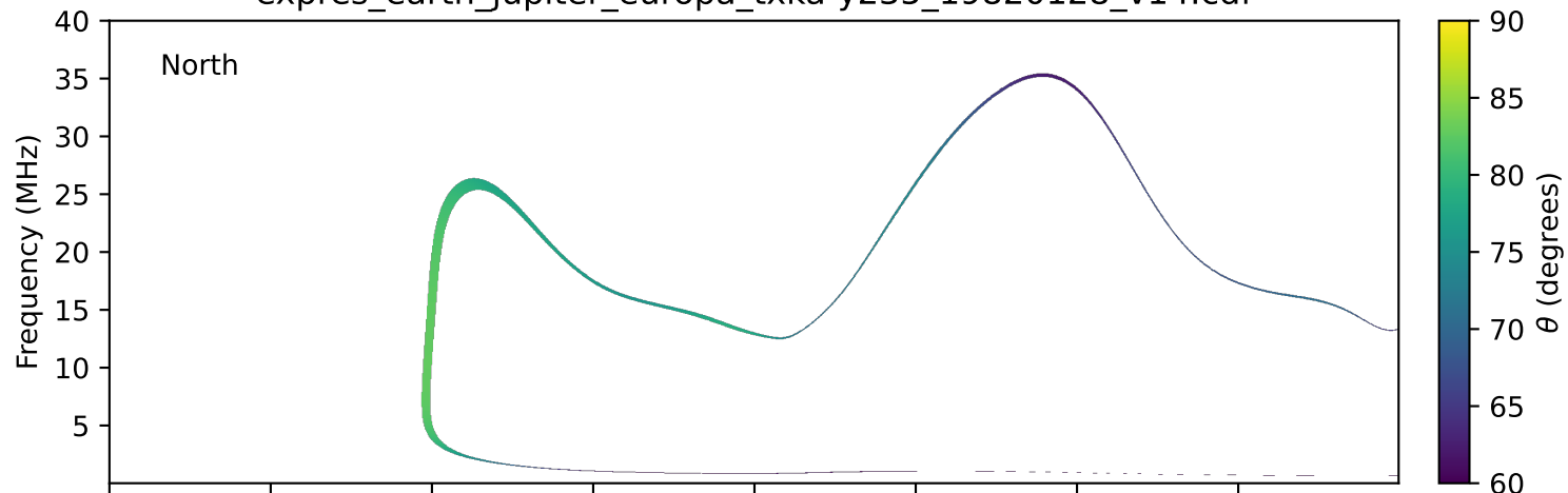
expres_earth_jupiter_europa_txka-y235_19820128_v14.cdf
