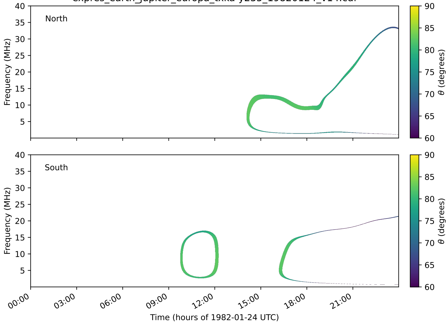
expres_earth_jupiter_europa_txka-y235_19820124_v14.cdf
