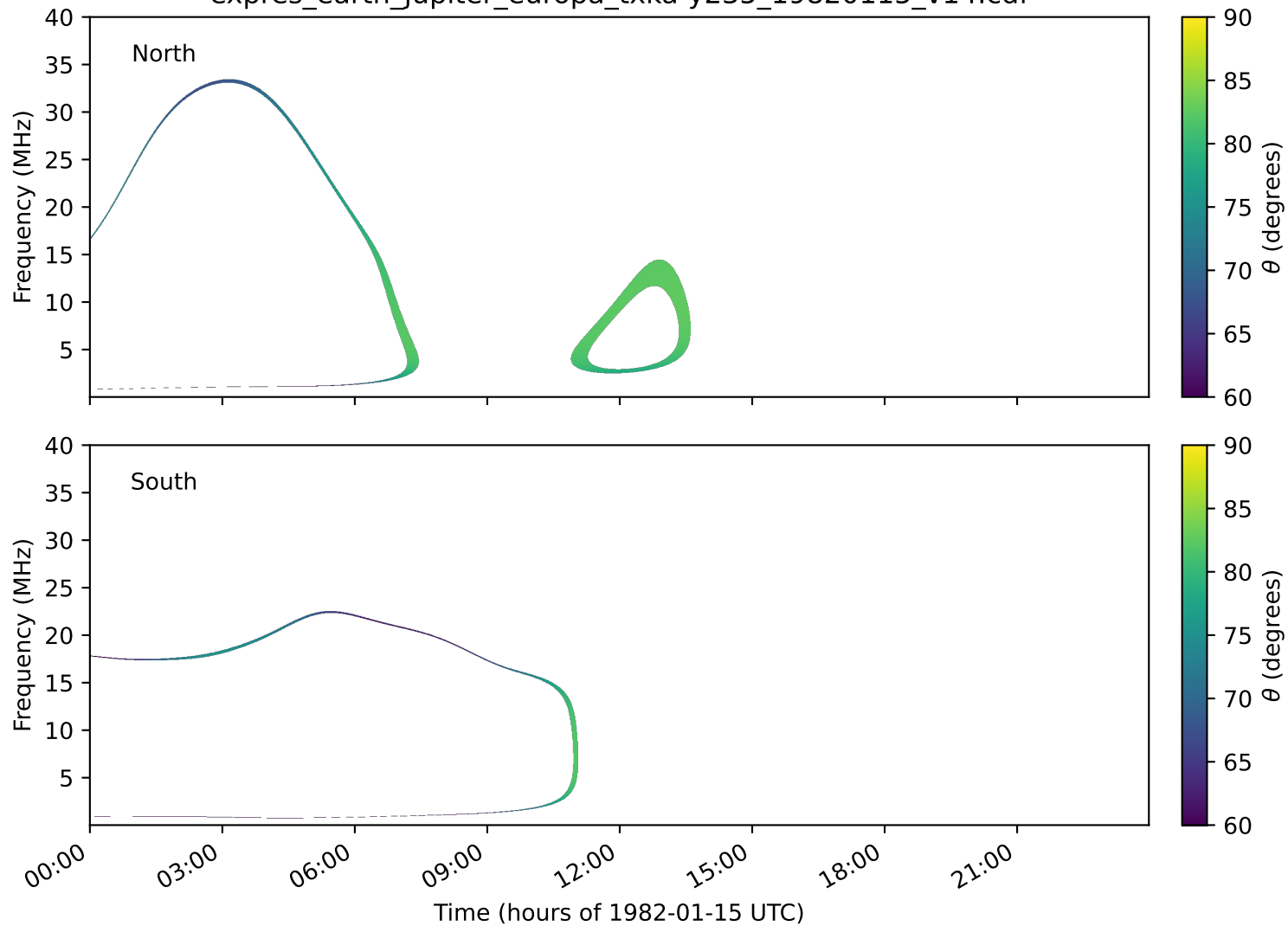
expres_earth_jupiter_europa_txka-y235_19820115_v14.cdf
