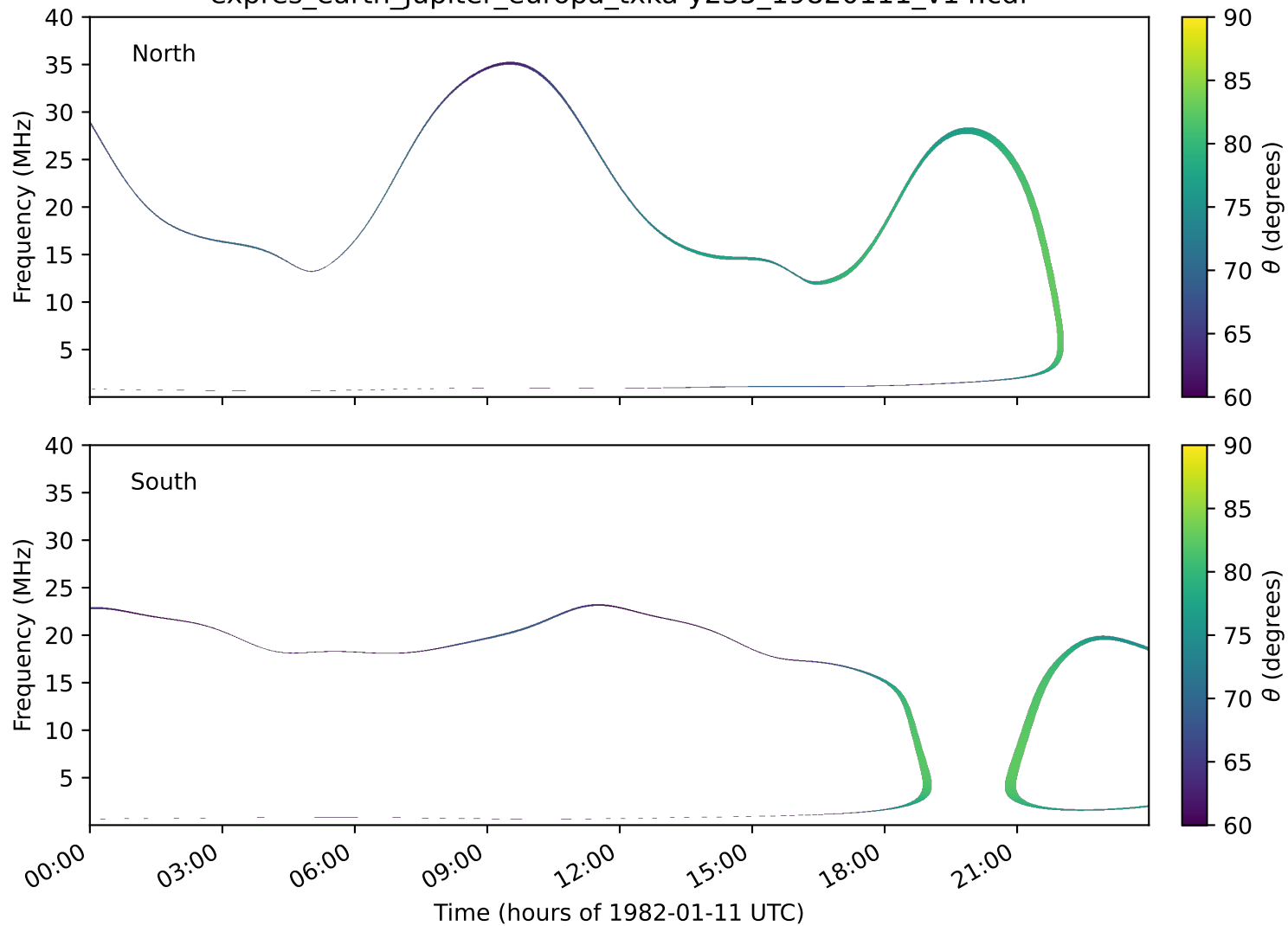
expres_earth_jupiter_europa_txka-y235_19820111_v14.cdf
