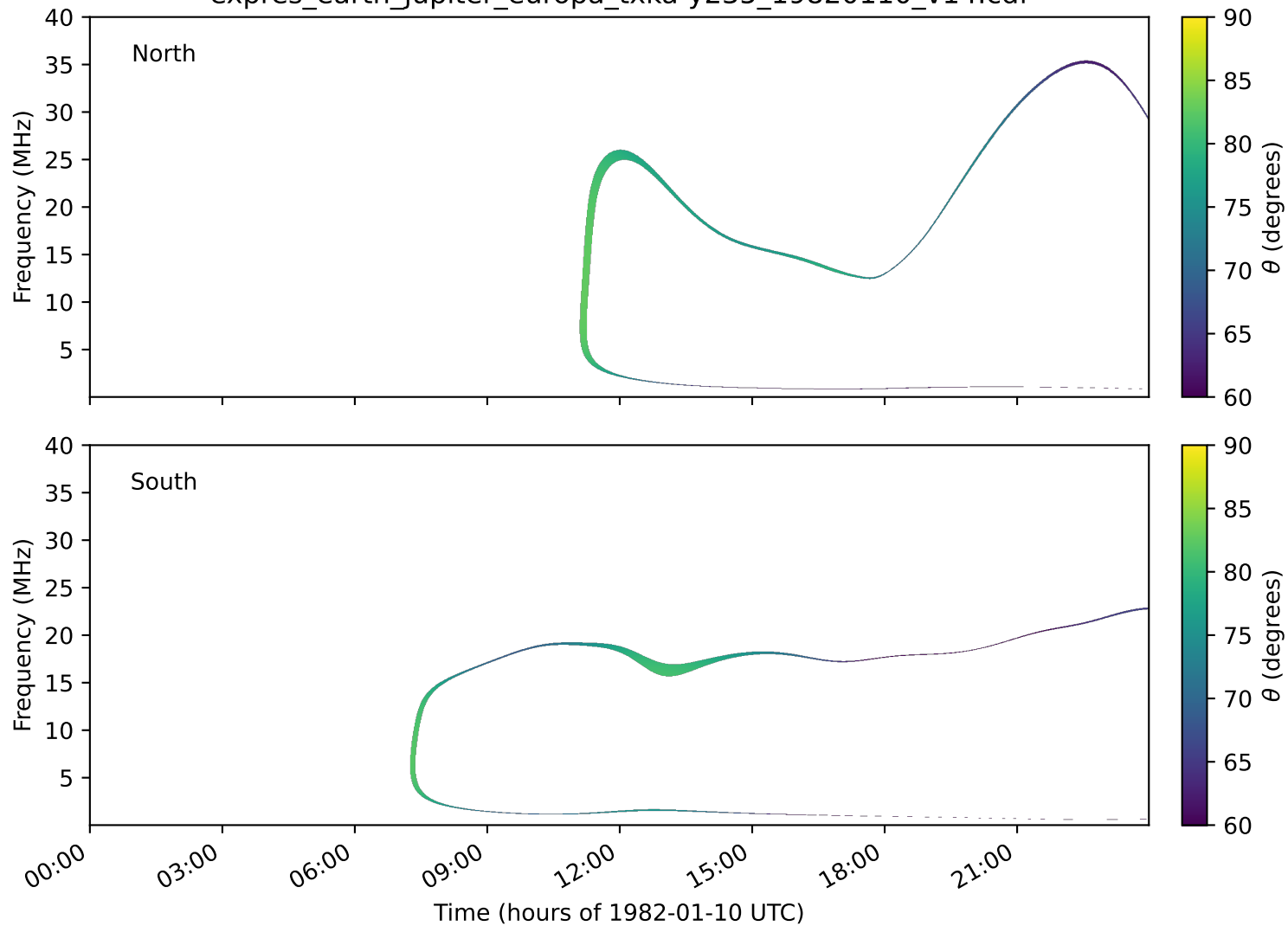
expres_earth_jupiter_europa_txka-y235_19820110_v14.cdf
