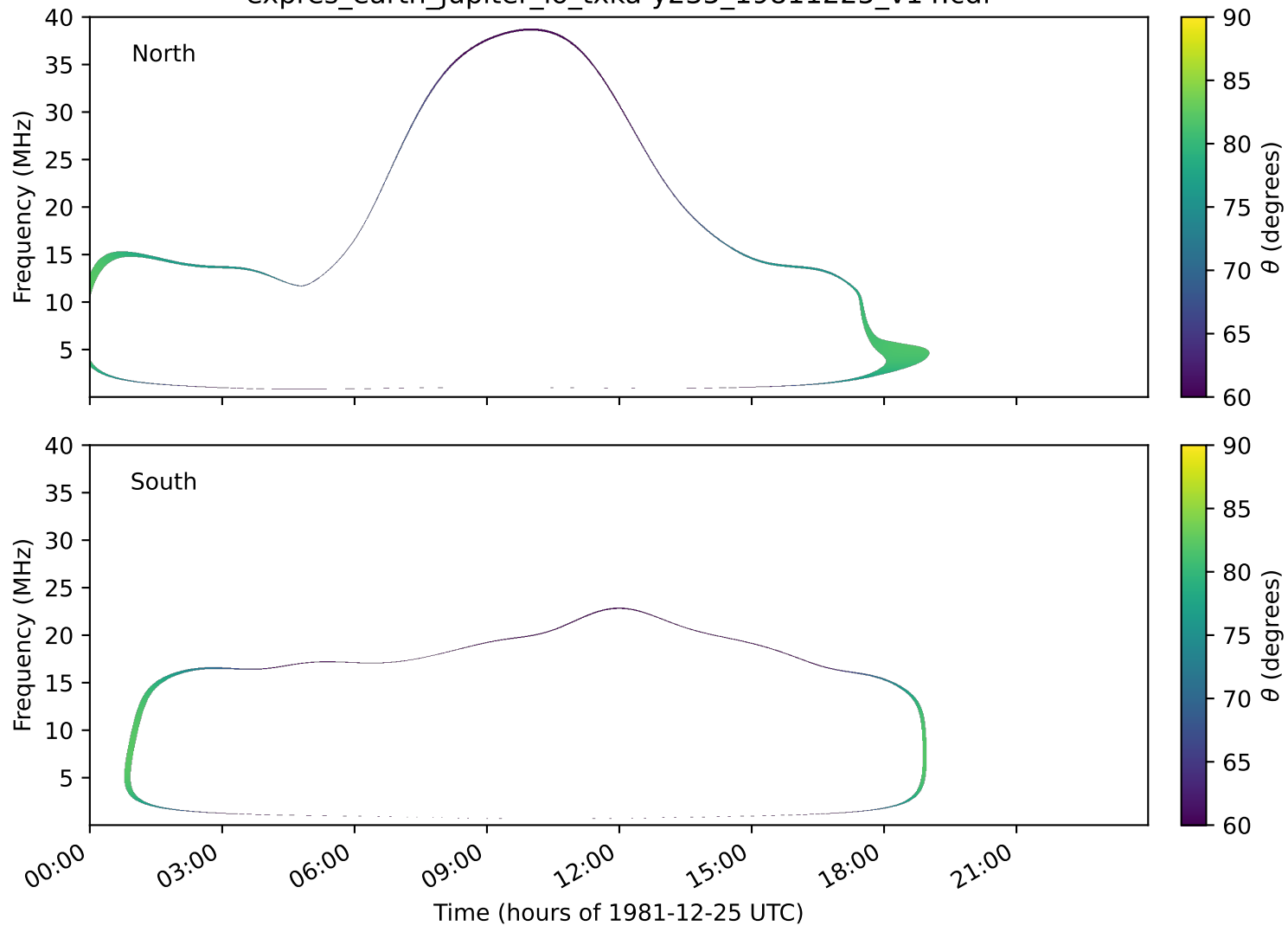
expres_earth_jupiter_io_txka-y235_19811225_v14.cdf
