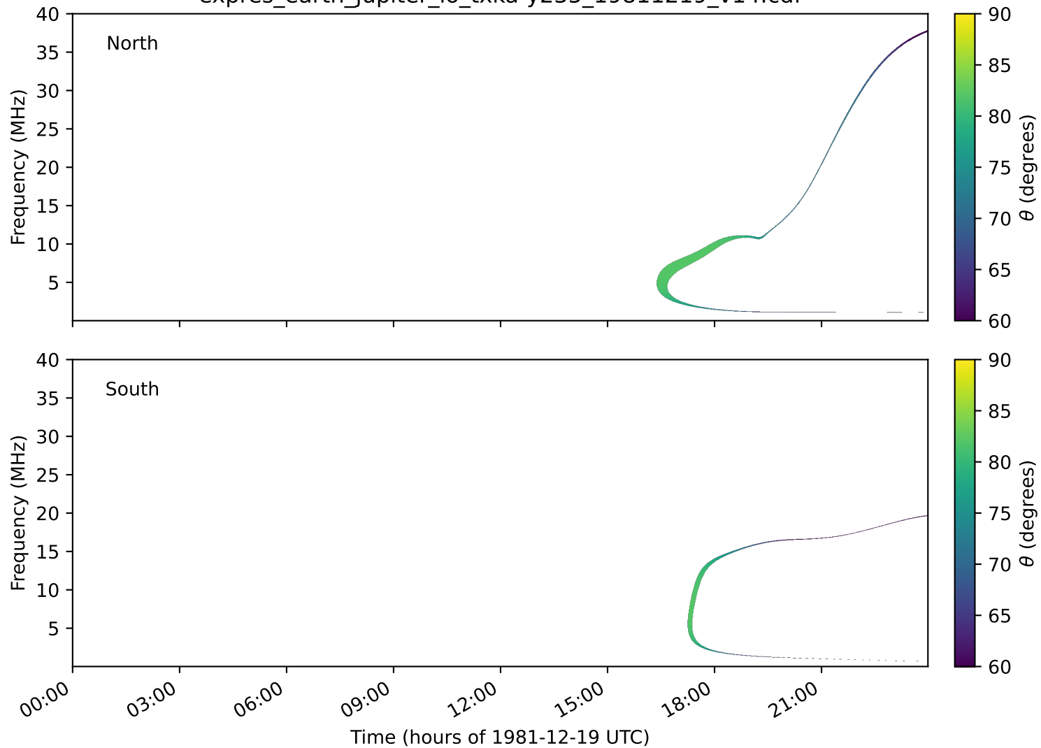
expres_earth_jupiter_io_txka-y235_19811219_v14.cdf
