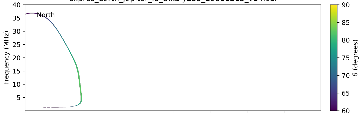
expres_earth_jupiter_io_txka-y235_19811213_v14.cdf
