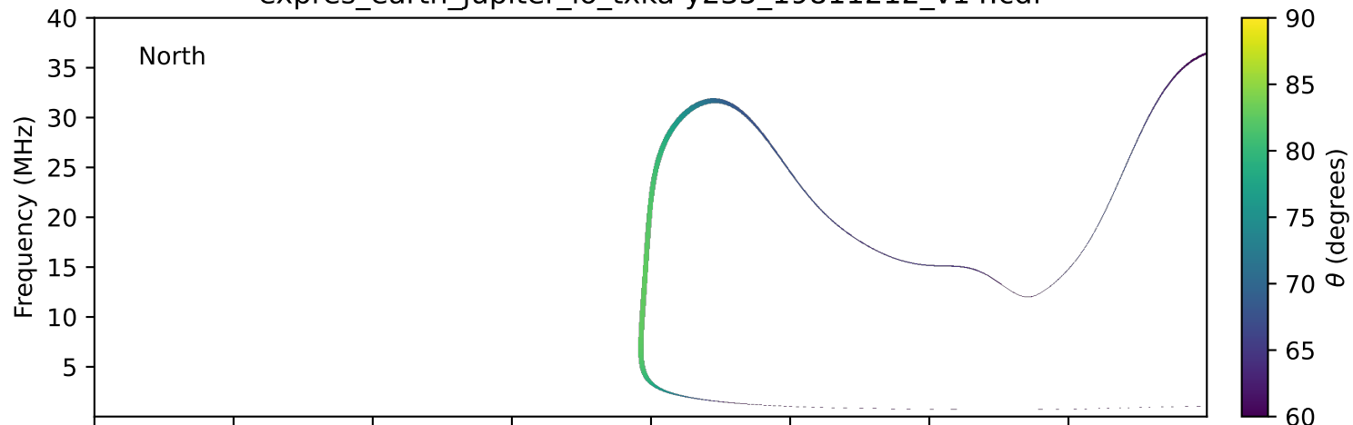
expres_earth_jupiter_io_txka-y235_19811212_v14.cdf
