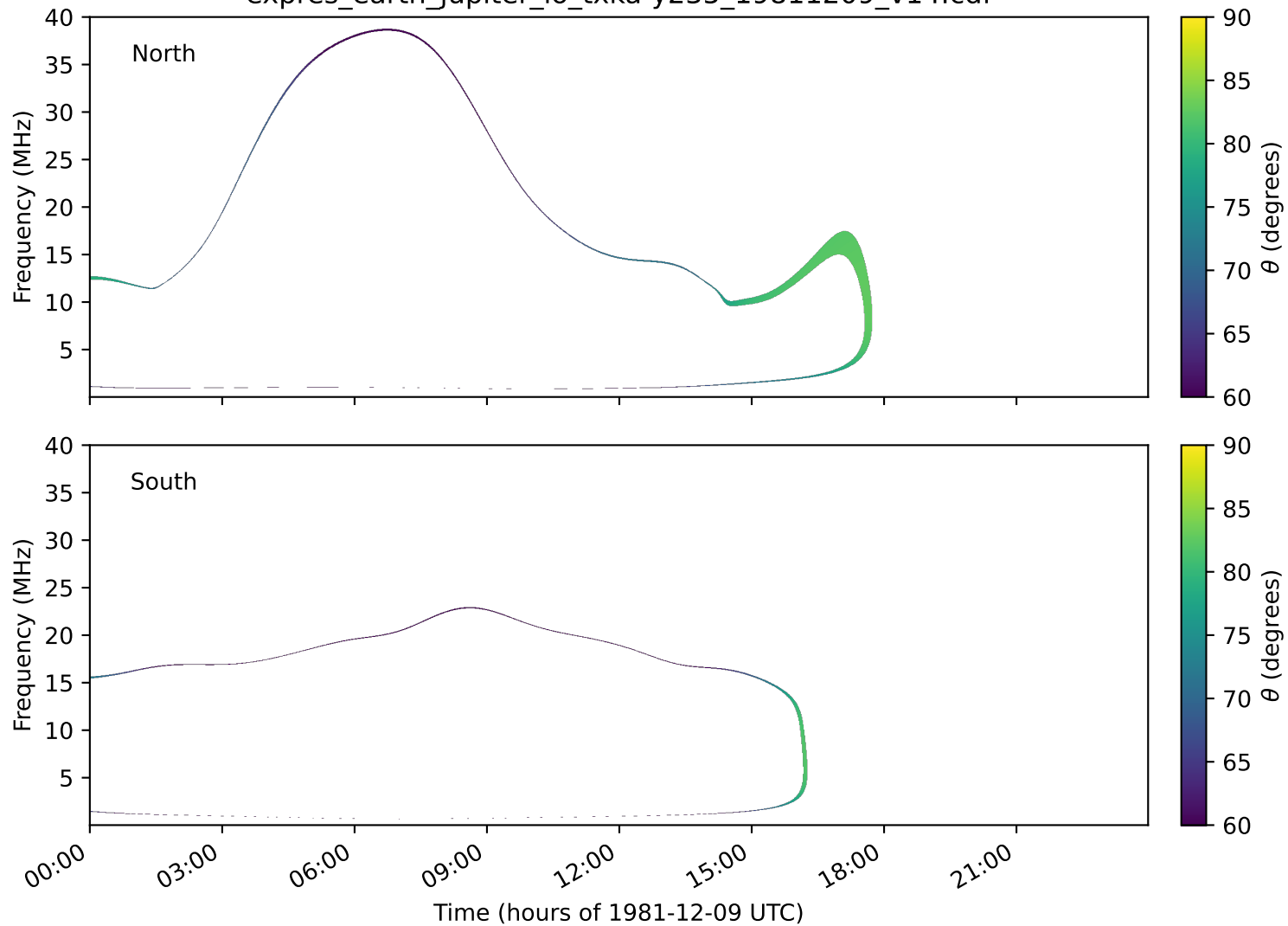
expres_earth_jupiter_io_txka-y235_19811209_v14.cdf
