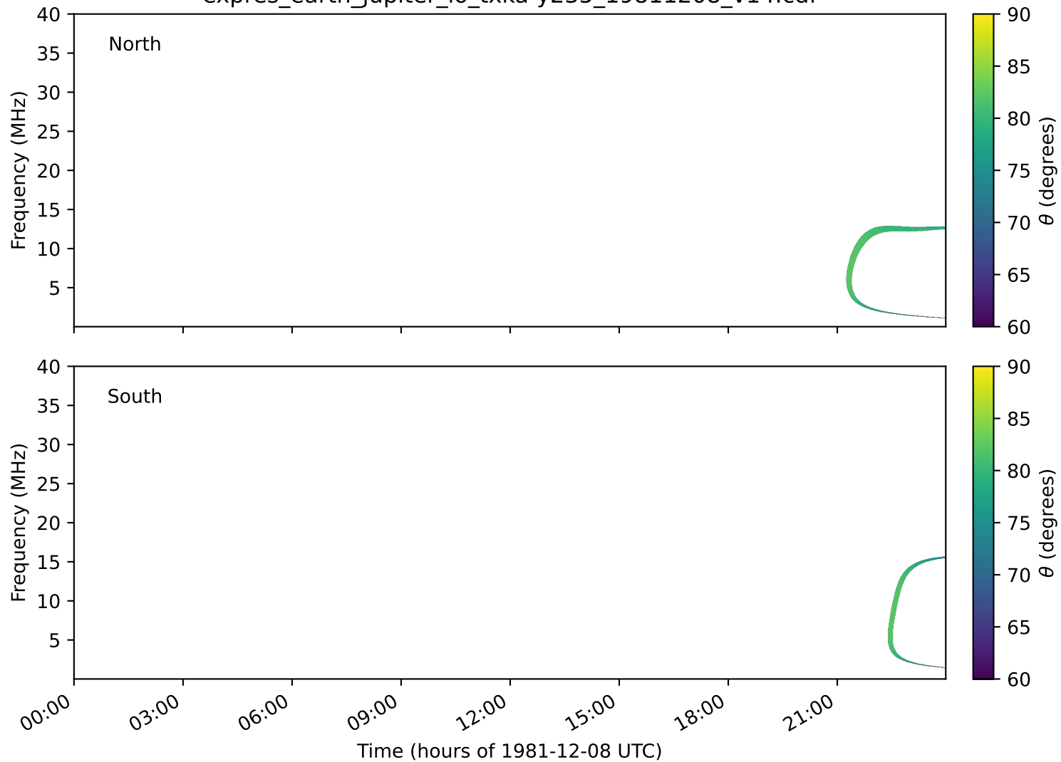
expres_earth_jupiter_io_txka-y235_19811208_v14.cdf
