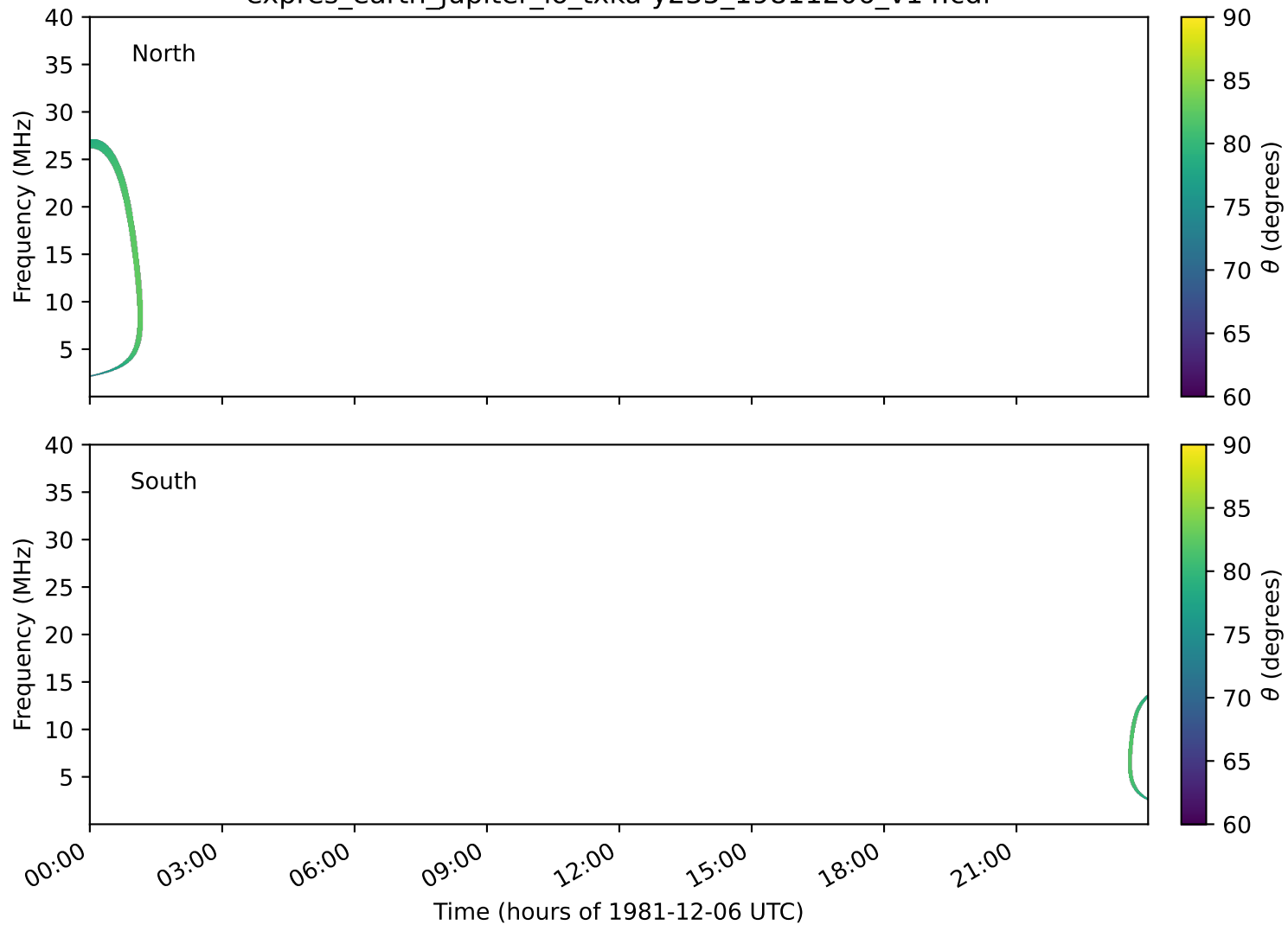
expres_earth_jupiter_io_txka-y235_19811206_v14.cdf
