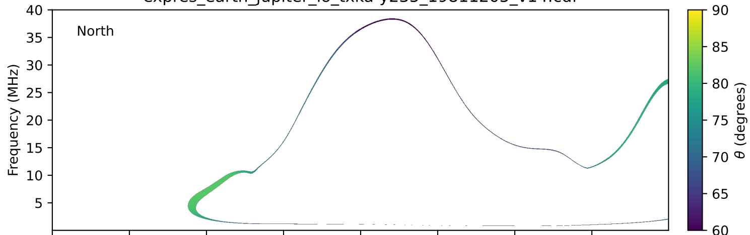
expres_earth_jupiter_io_txka-y235_19811205_v14.cdf
