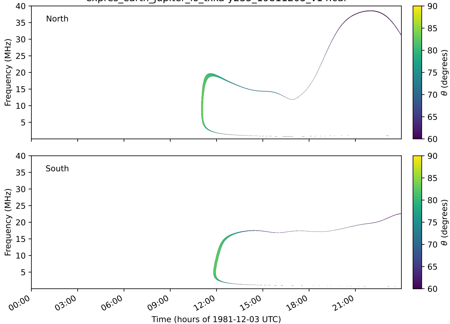
expres_earth_jupiter_io_txka-y235_19811203_v14.cdf
