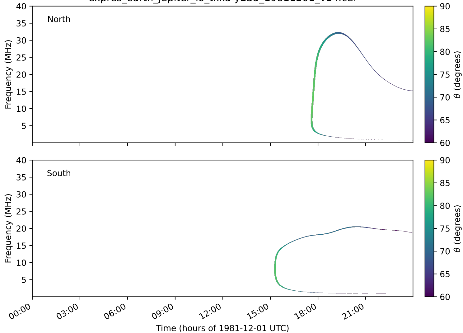
expres_earth_jupiter_io_txka-y235_19811201_v14.cdf
