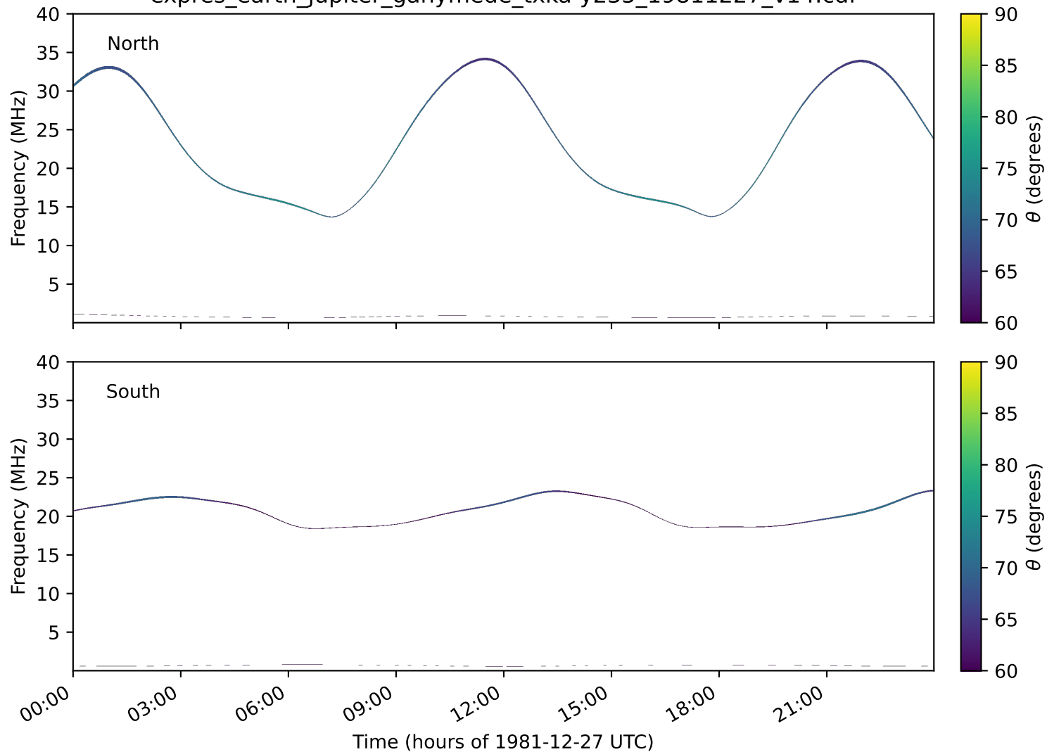
expres_earth_jupiter_ganymede_txka-y235_19811227_v14.cdf
