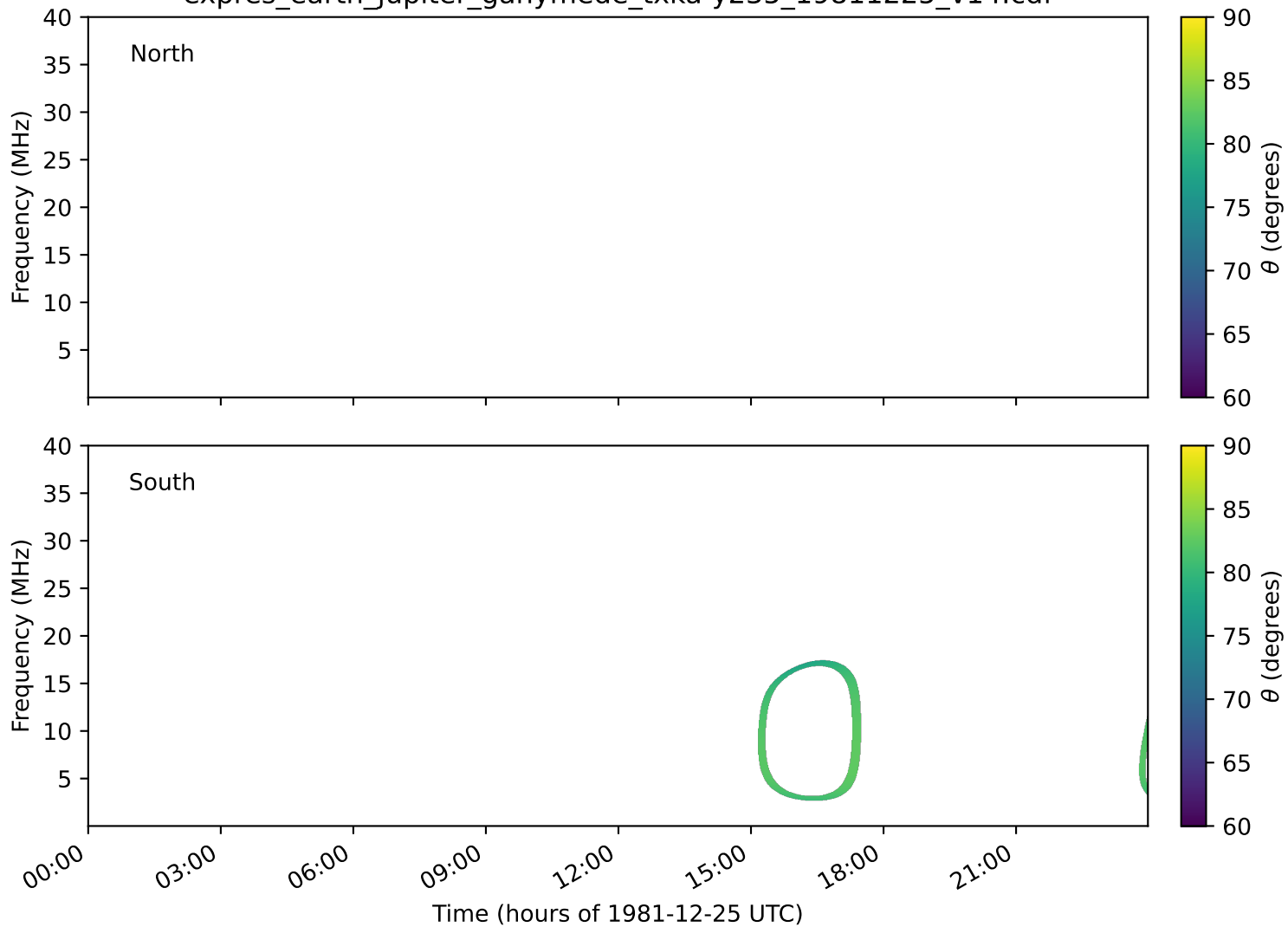
expres_earth_jupiter_ganymede_txka-y235_19811225_v14.cdf
