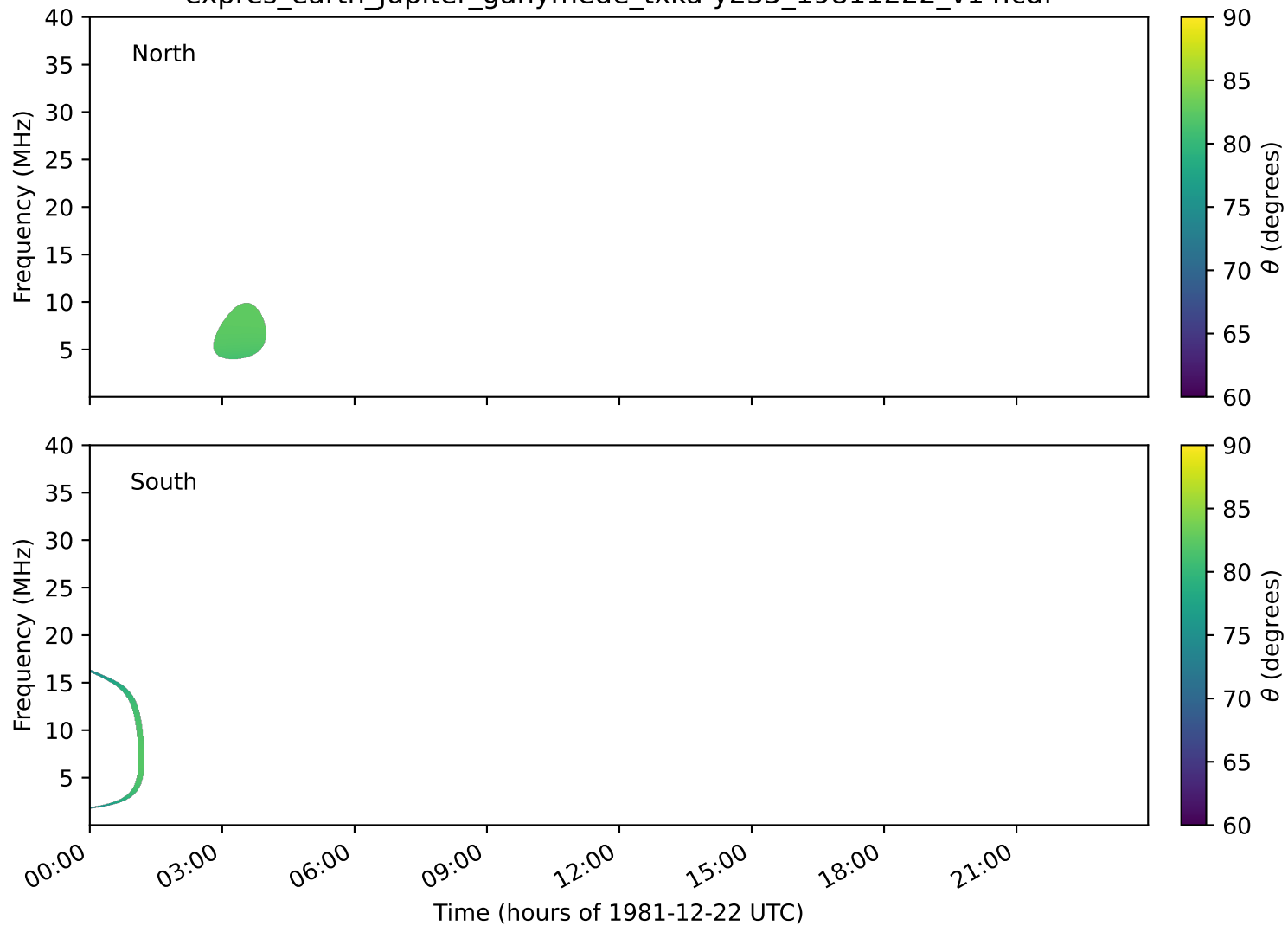
expres_earth_jupiter_ganymede_txka-y235_19811222_v14.cdf
