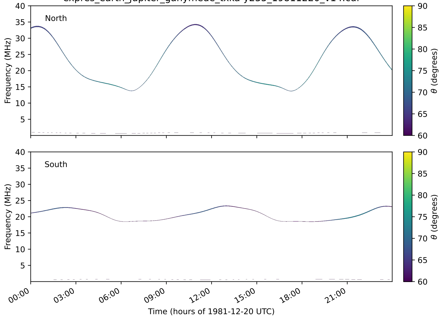
expres_earth_jupiter_ganymede_txka-y235_19811220_v14.cdf
