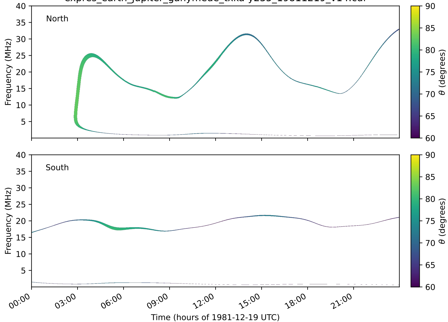
expres_earth_jupiter_ganymede_txka-y235_19811219_v14.cdf
