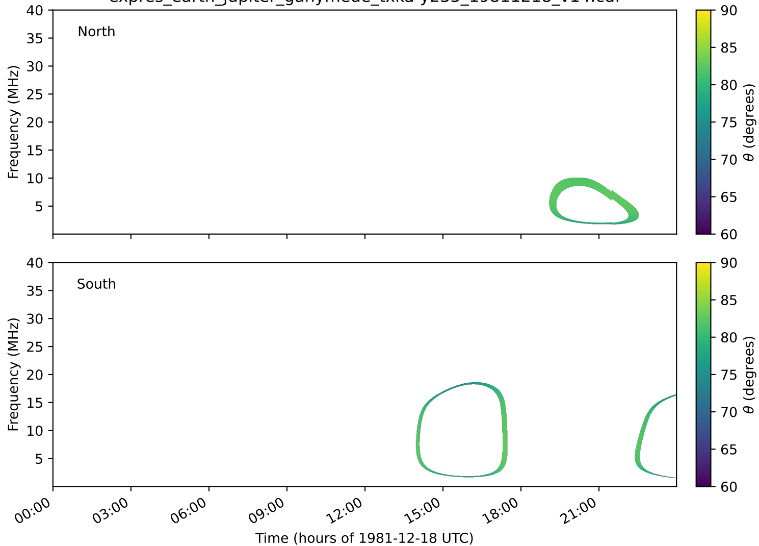
expres_earth_jupiter_ganymede_txka-y235_19811218_v14.cdf
