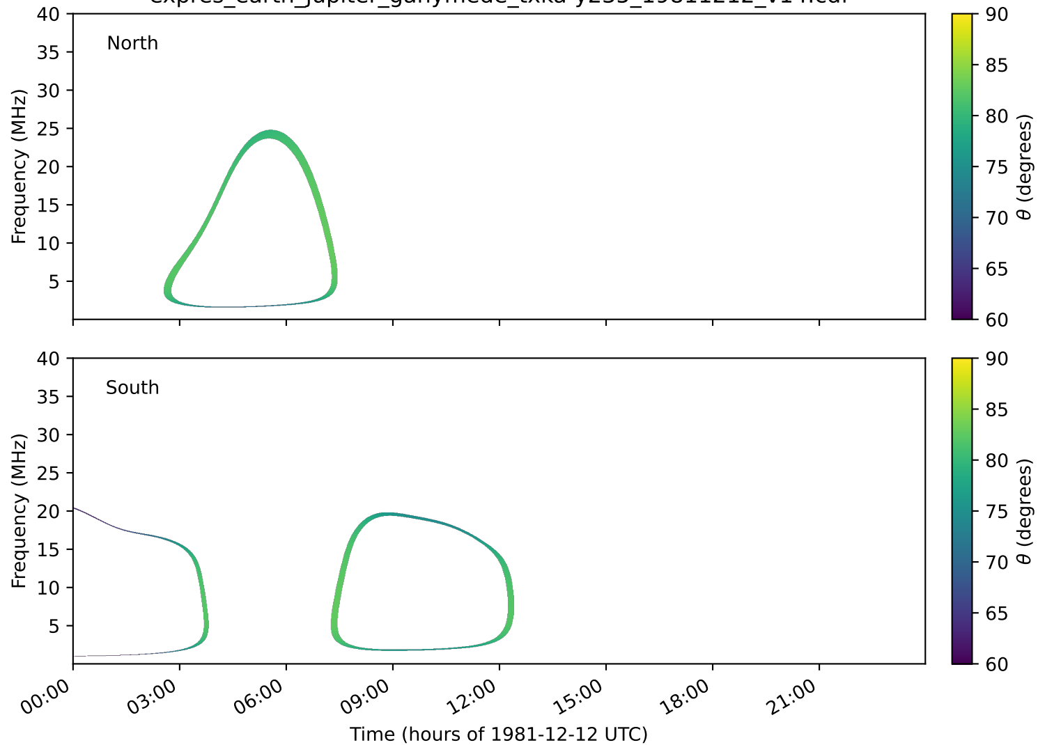
expres_earth_jupiter_ganymede_txka-y235_19811212_v14.cdf
