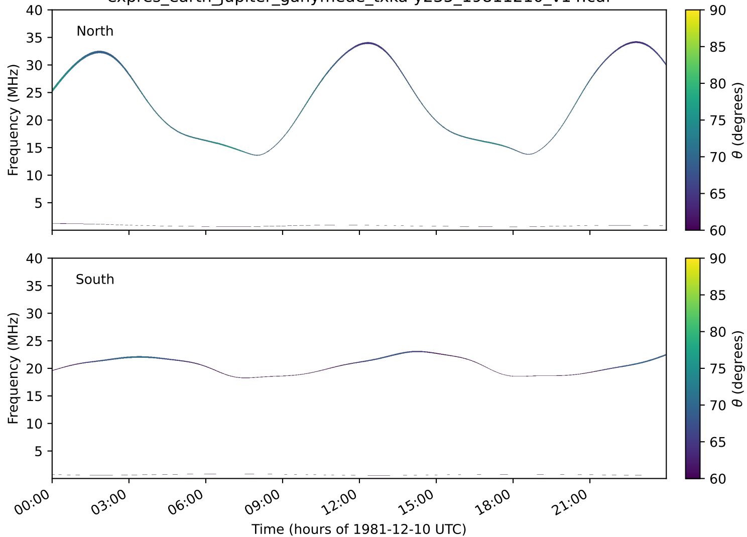
expres_earth_jupiter_ganymede_txka-y235_19811210_v14.cdf
