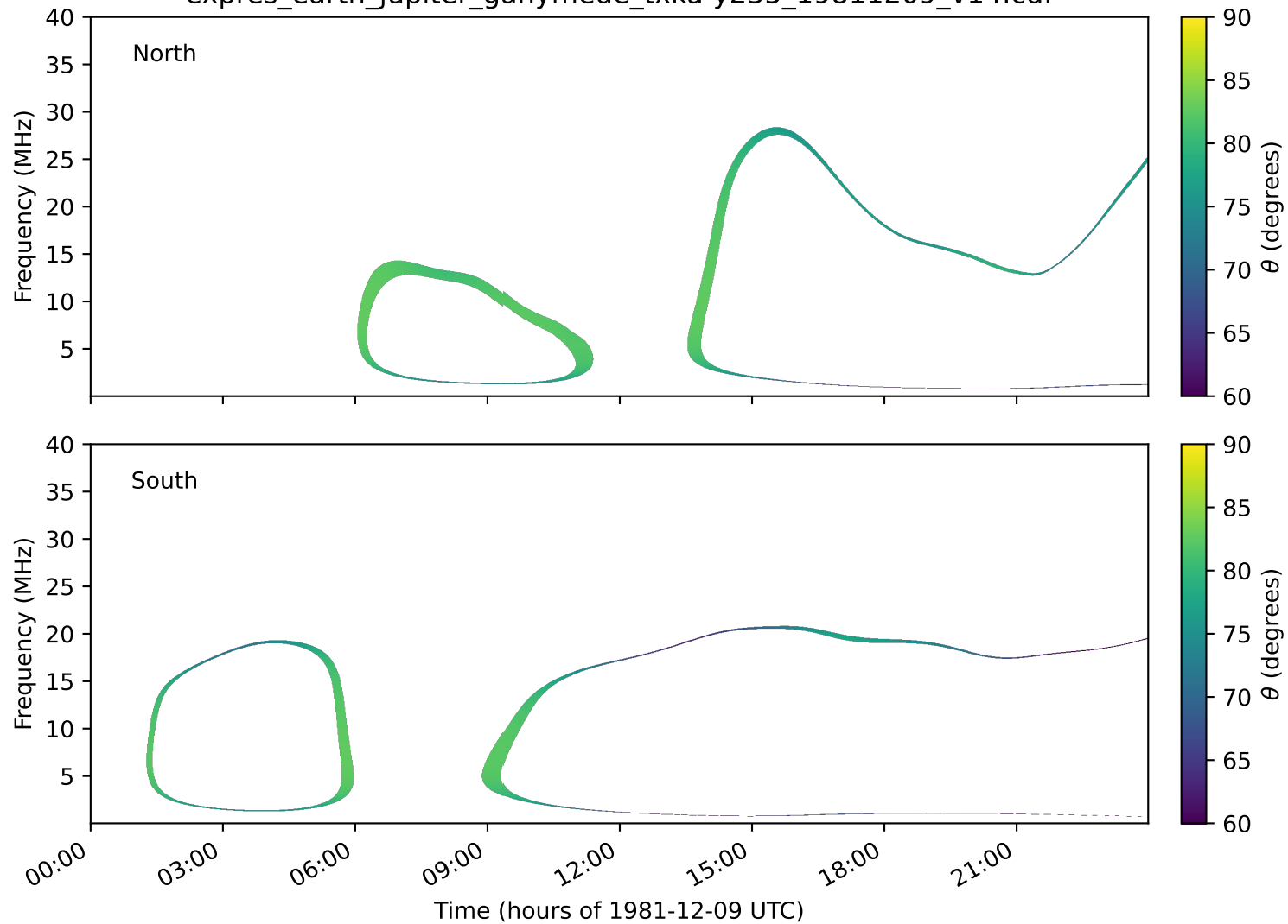
expres_earth_jupiter_ganymede_txka-y235_19811209_v14.cdf
