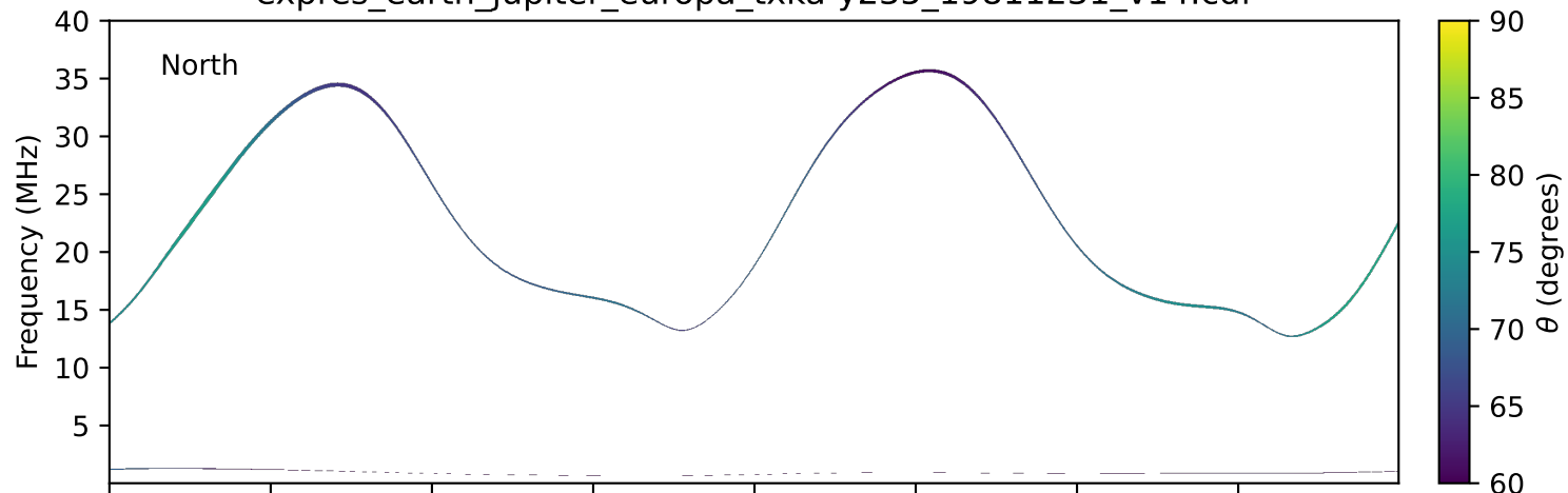
expres_earth_jupiter_europa_txka-y235_19811231_v14.cdf
