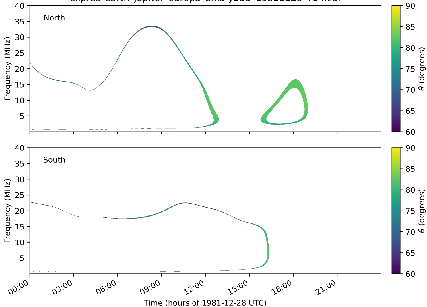
expres_earth_jupiter_europa_txka-y235_19811228_v14.cdf
