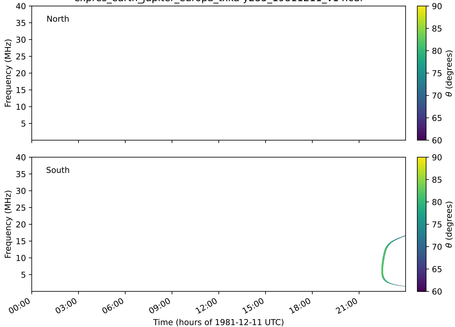
expres_earth_jupiter_europa_txka-y235_19811211_v14.cdf
