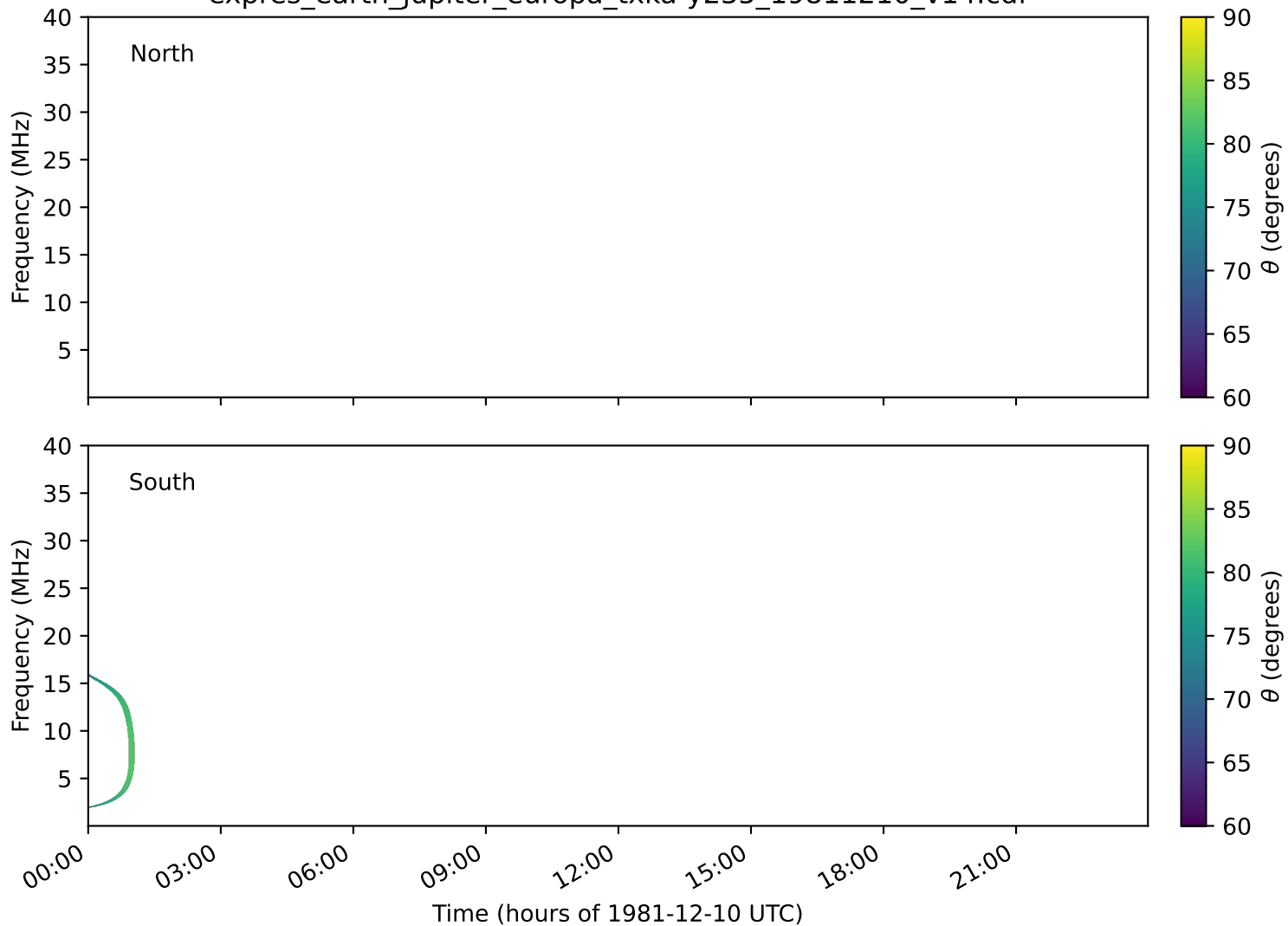
expres_earth_jupiter_europa_txka-y235_19811210_v14.cdf
