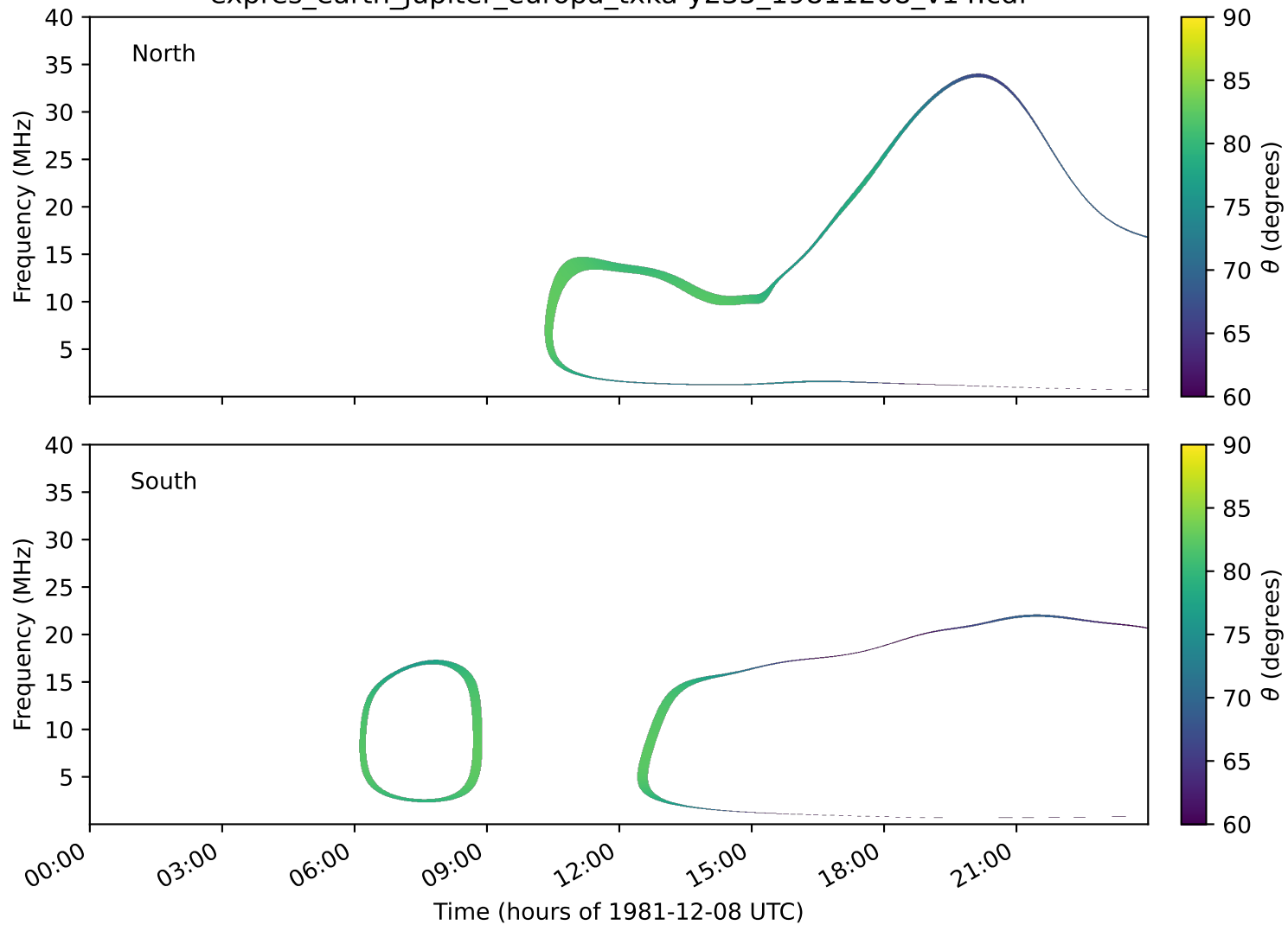
expres_earth_jupiter_europa_txka-y235_19811208_v14.cdf
