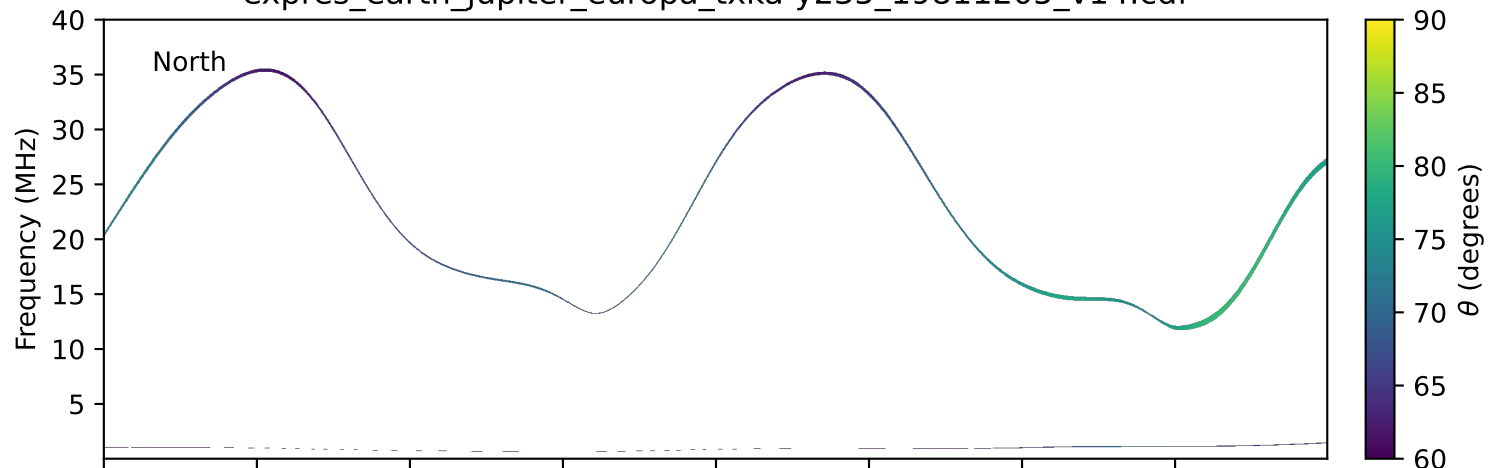
expres_earth_jupiter_europa_txka-y235_19811205_v14.cdf
