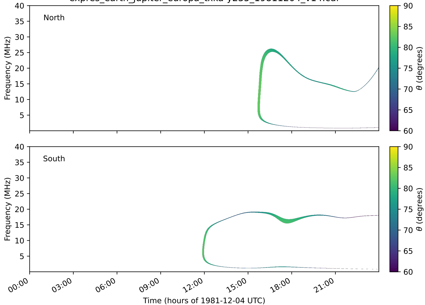
expres_earth_jupiter_europa_txka-y235_19811204_v14.cdf
