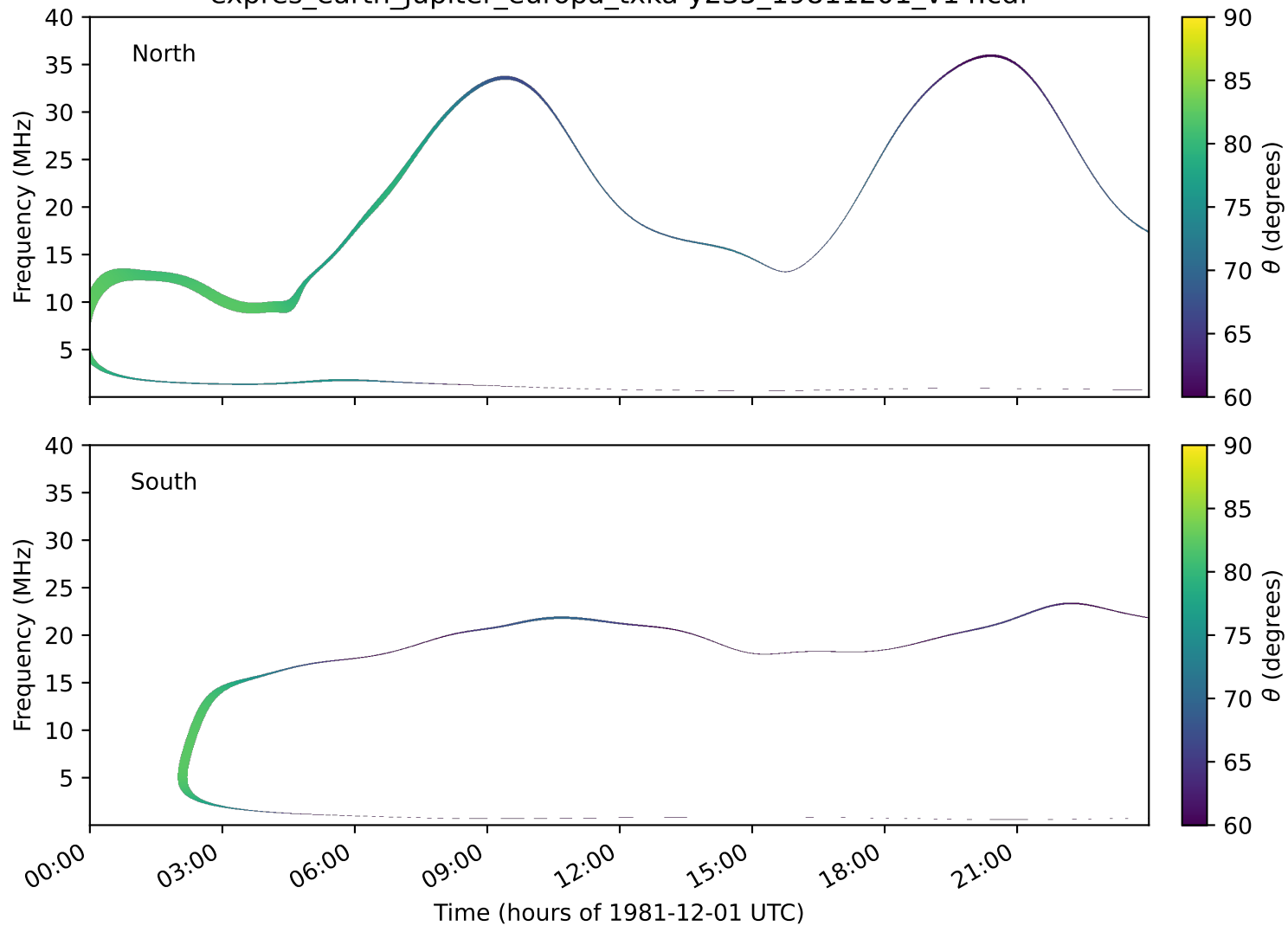
expres_earth_jupiter_europa_txka-y235_19811201_v14.cdf
