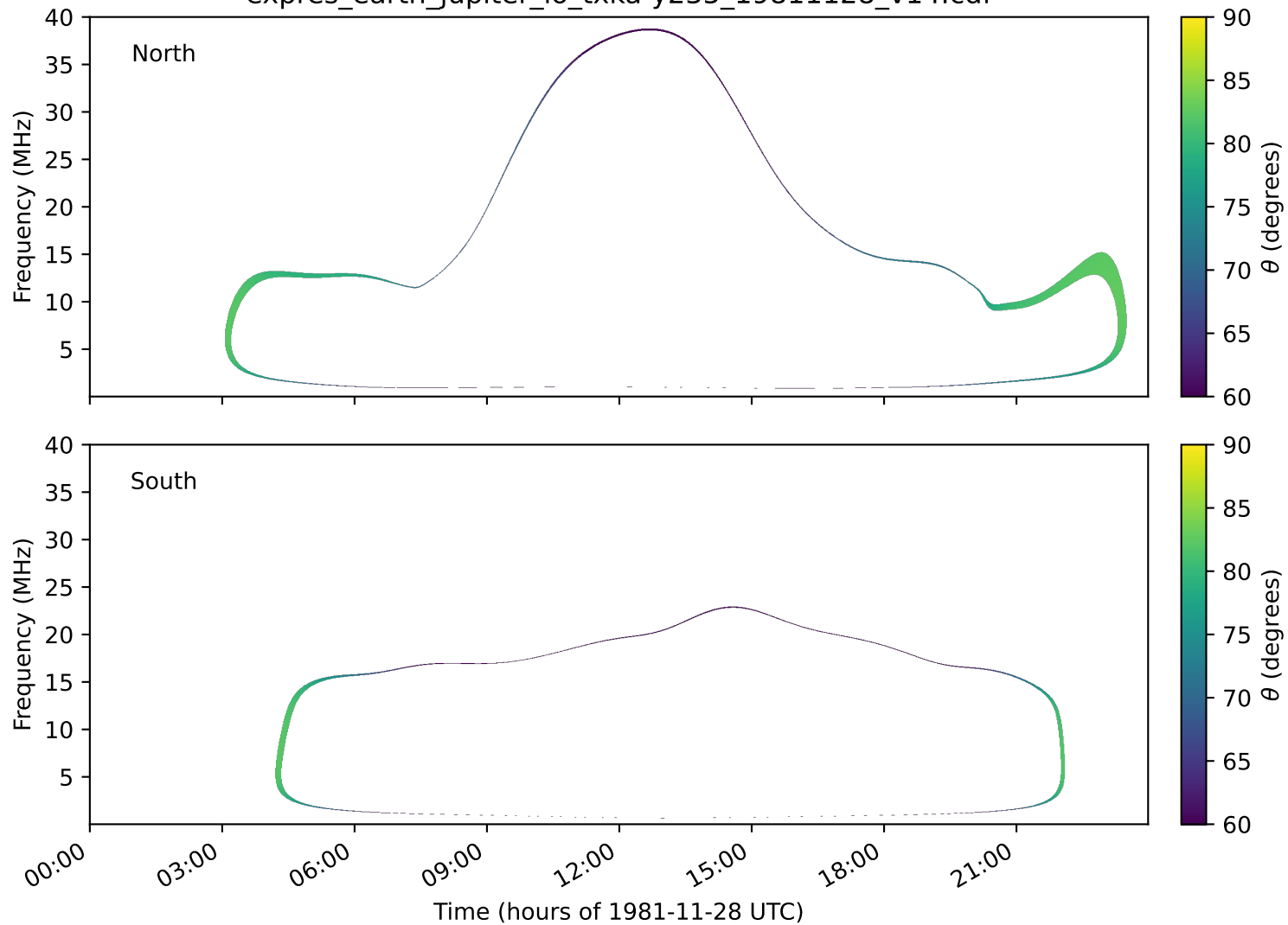
expres_earth_jupiter_io_txka-y235_19811128_v14.cdf
