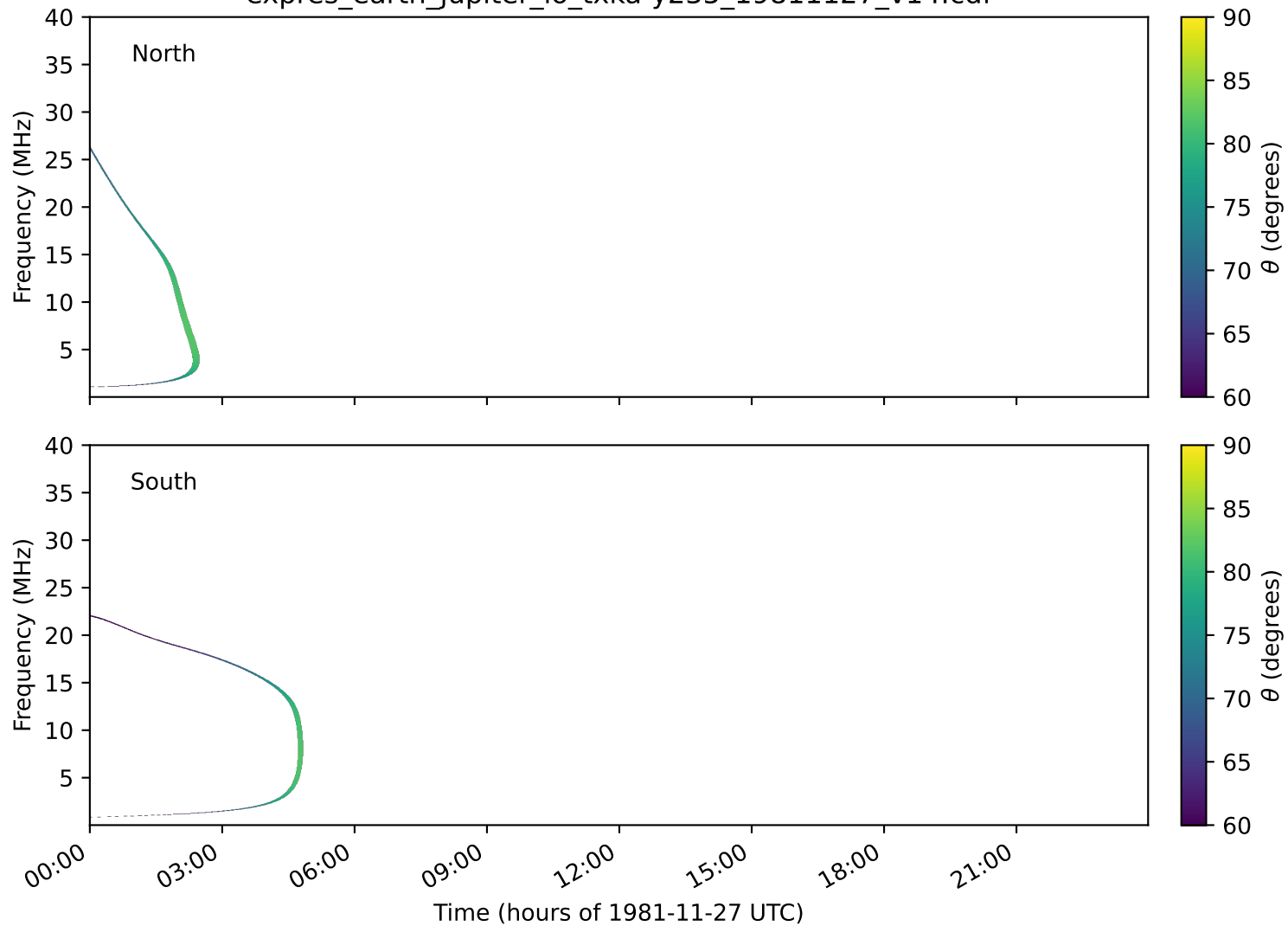
expres_earth_jupiter_io_txka-y235_19811127_v14.cdf
