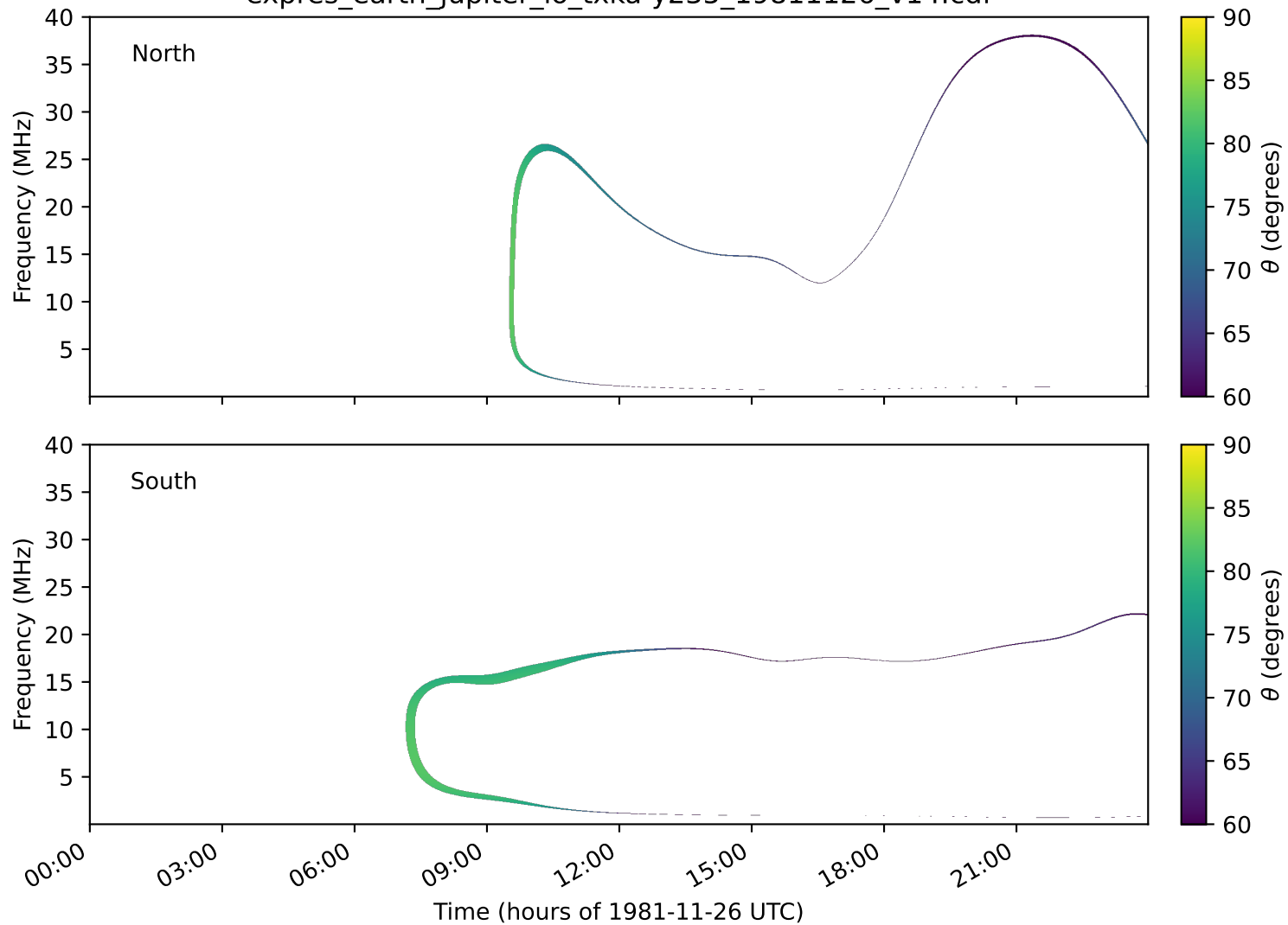
expres_earth_jupiter_io_txka-y235_19811126_v14.cdf
