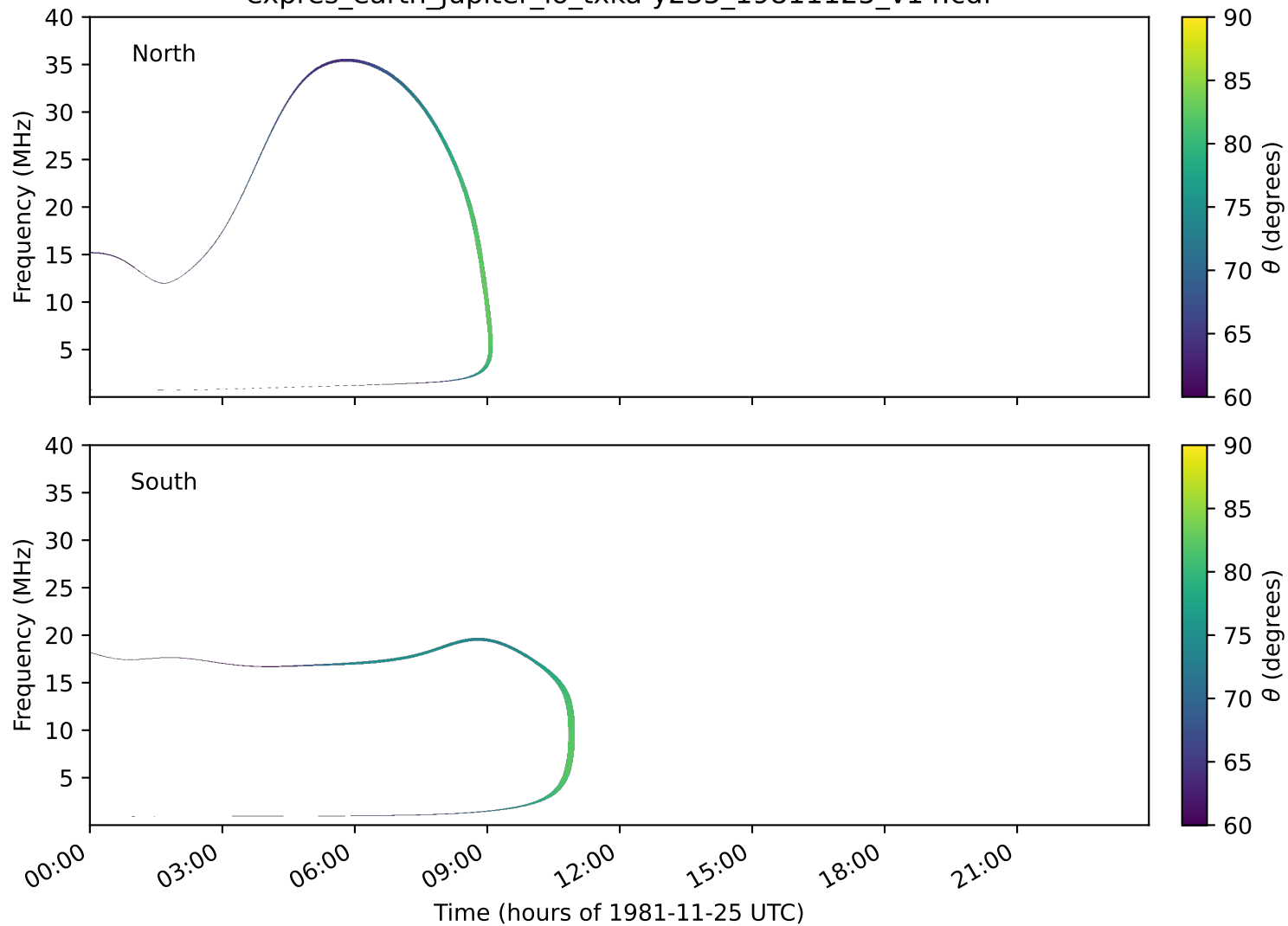
expres_earth_jupiter_io_txka-y235_19811125_v14.cdf
