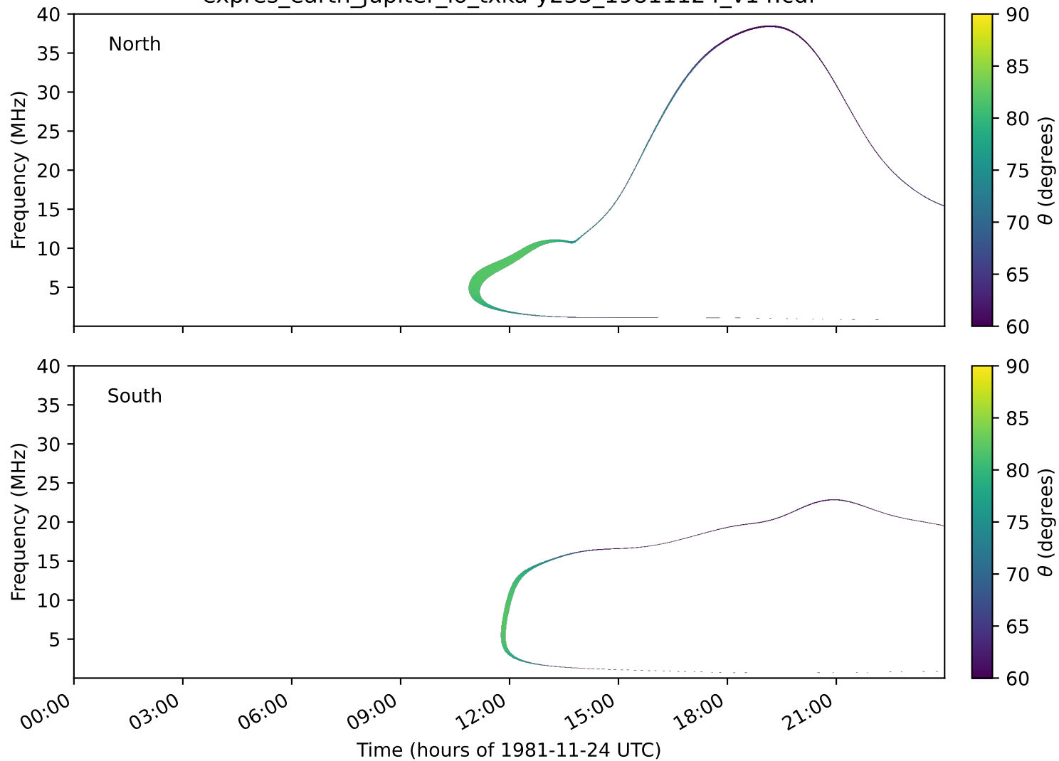
expres_earth_jupiter_io_txka-y235_19811124_v14.cdf
