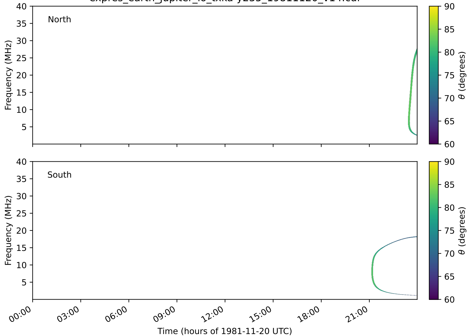
expres_earth_jupiter_io_txka-y235_19811120_v14.cdf
