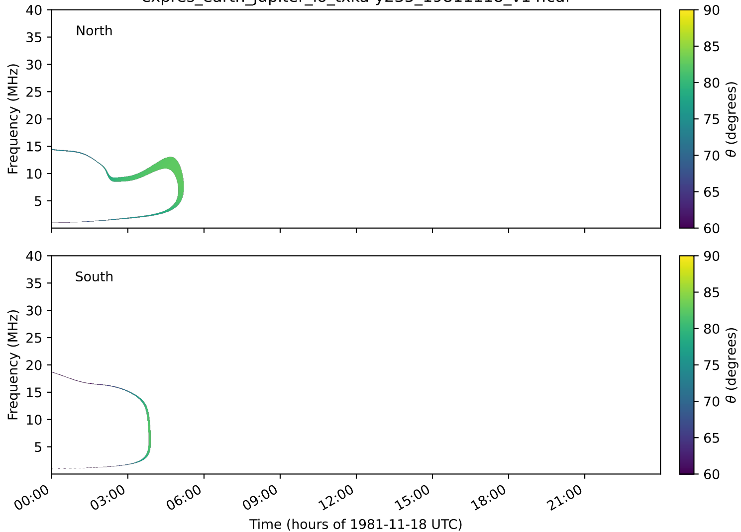
expres_earth_jupiter_io_txka-y235_19811118_v14.cdf
