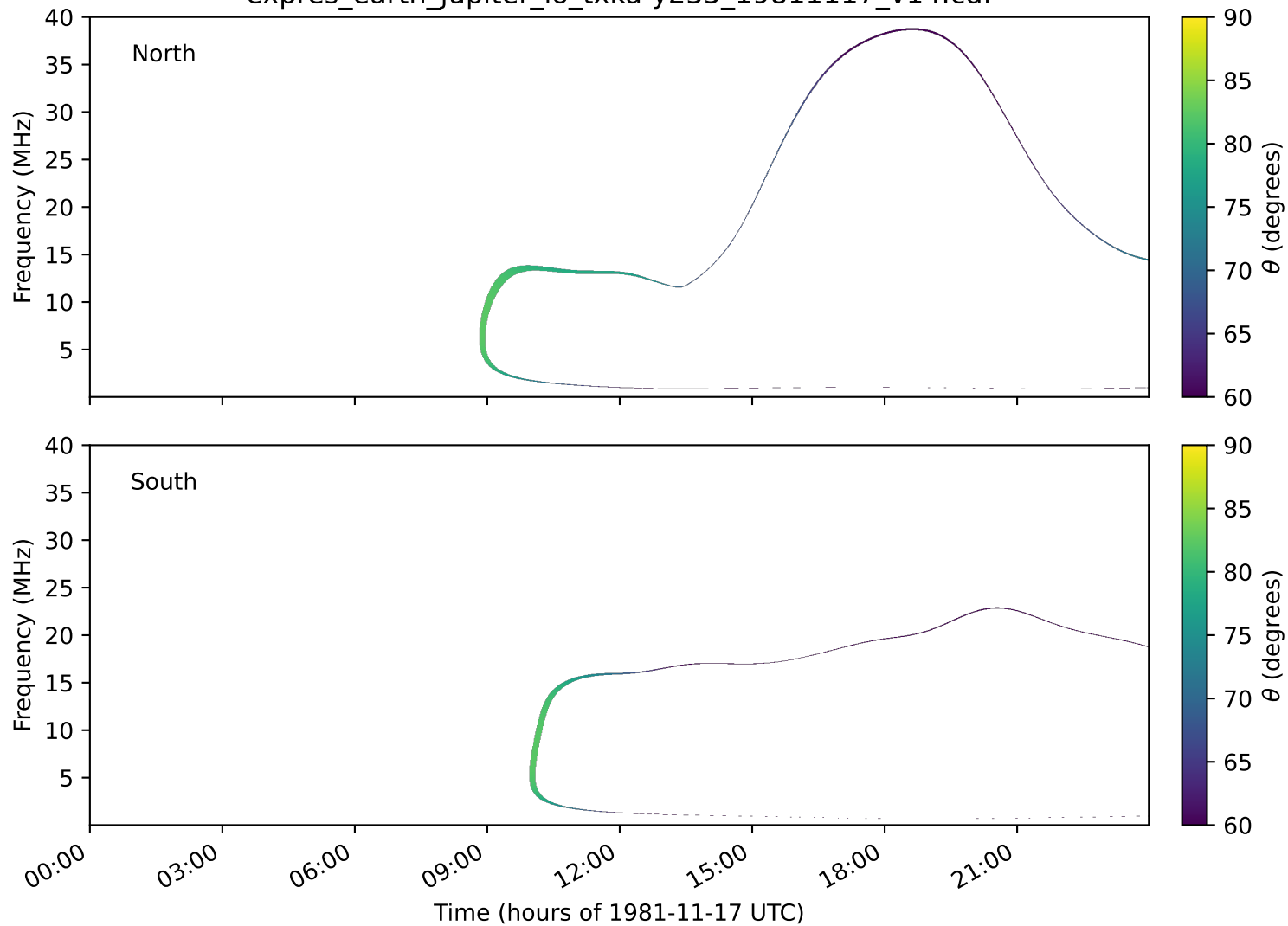
expres_earth_jupiter_io_txka-y235_19811117_v14.cdf
