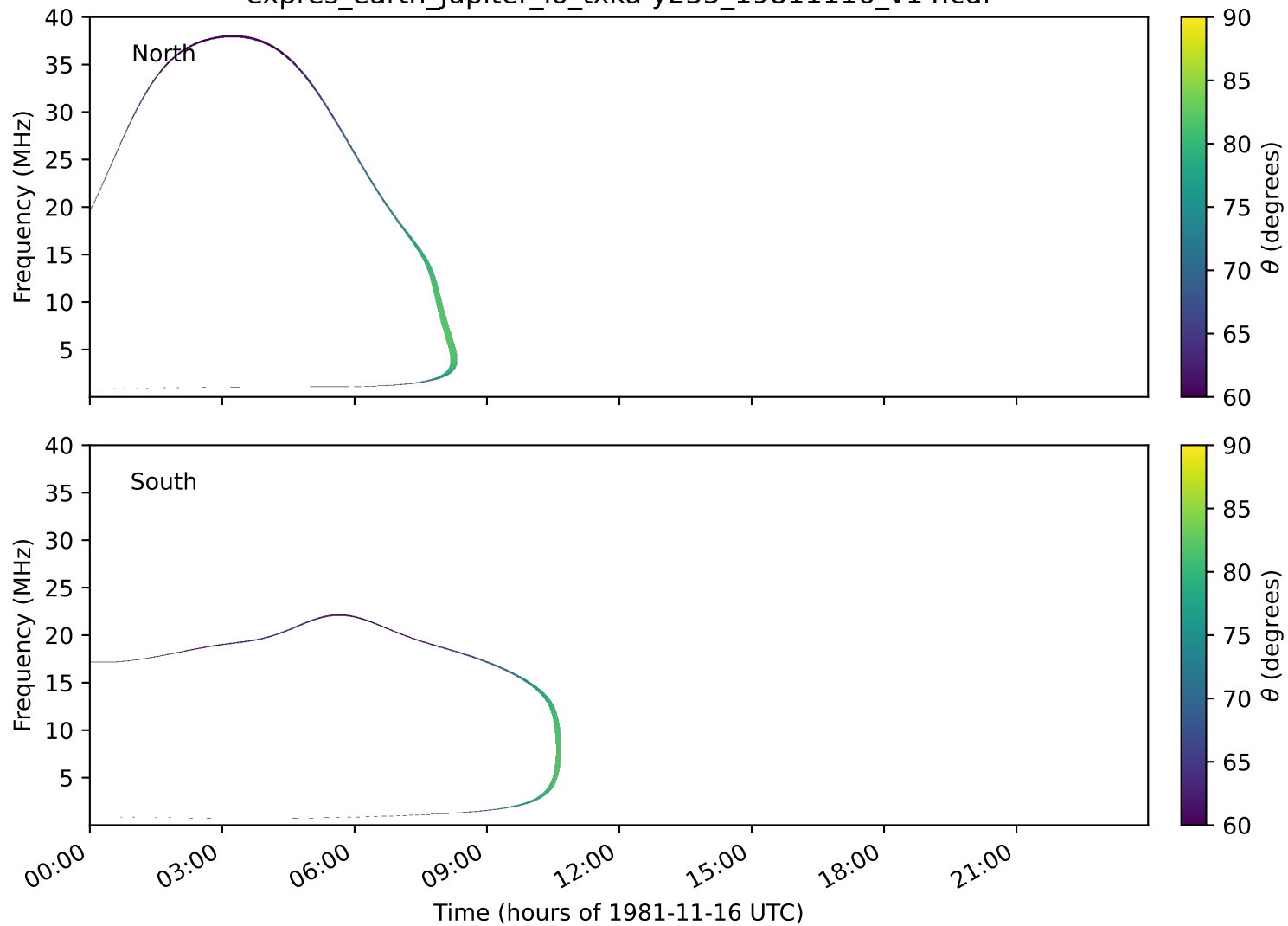
expres_earth_jupiter_io_txka-y235_19811116_v14.cdf
