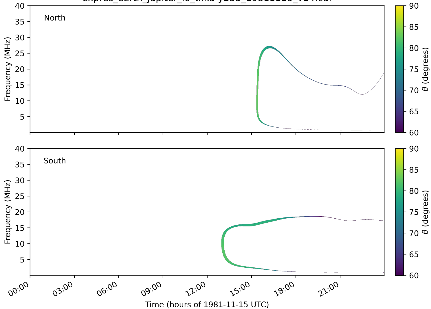
expres_earth_jupiter_io_txka-y235_19811115_v14.cdf
