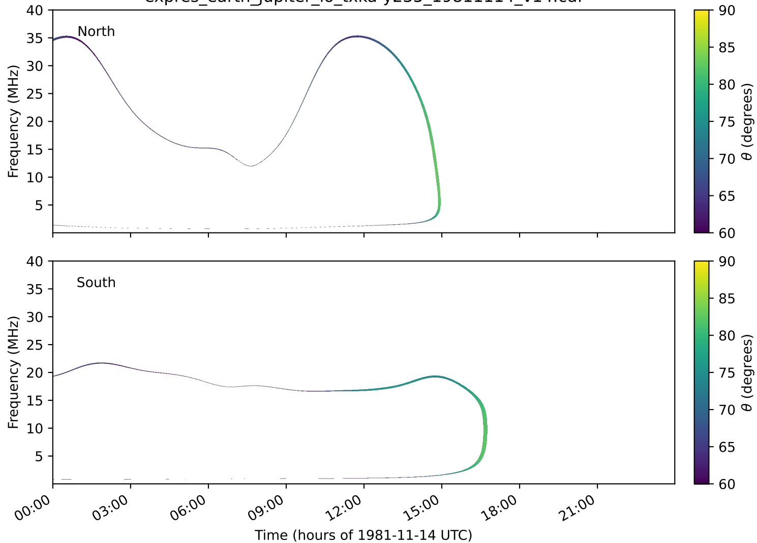
expres_earth_jupiter_io_txka-y235_19811114_v14.cdf
