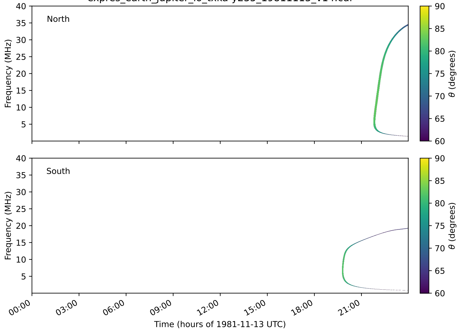
expres_earth_jupiter_io_txka-y235_19811113_v14.cdf
