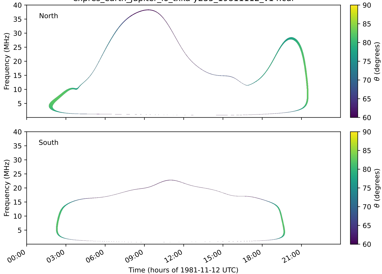
expres_earth_jupiter_io_txka-y235_19811112_v14.cdf
