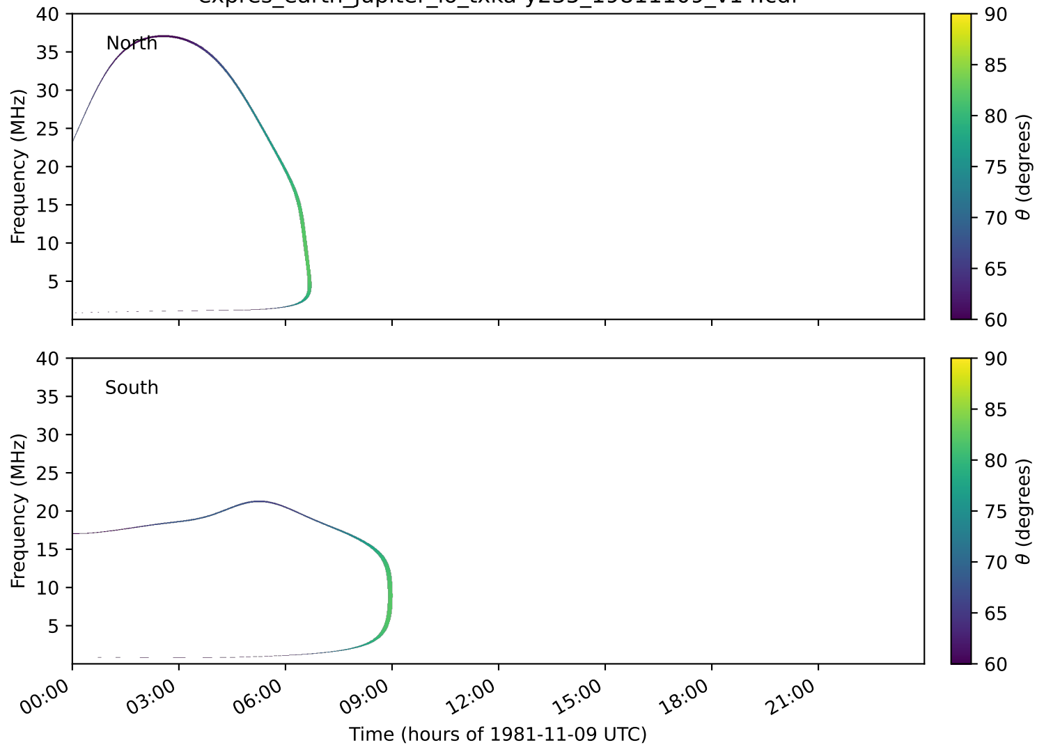
expres_earth_jupiter_io_txka-y235_19811109_v14.cdf
