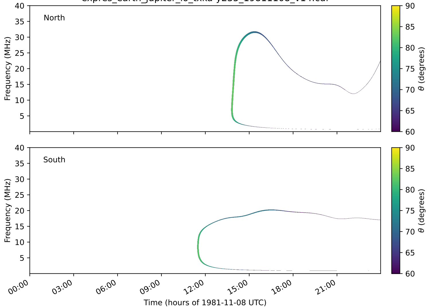
expres_earth_jupiter_io_txka-y235_19811108_v14.cdf
