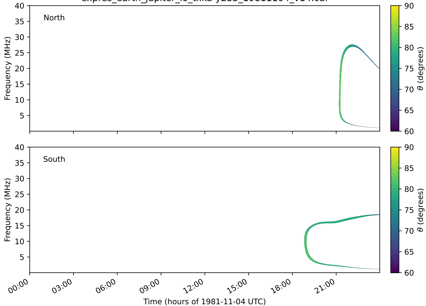
expres_earth_jupiter_io_txka-y235_19811104_v14.cdf
