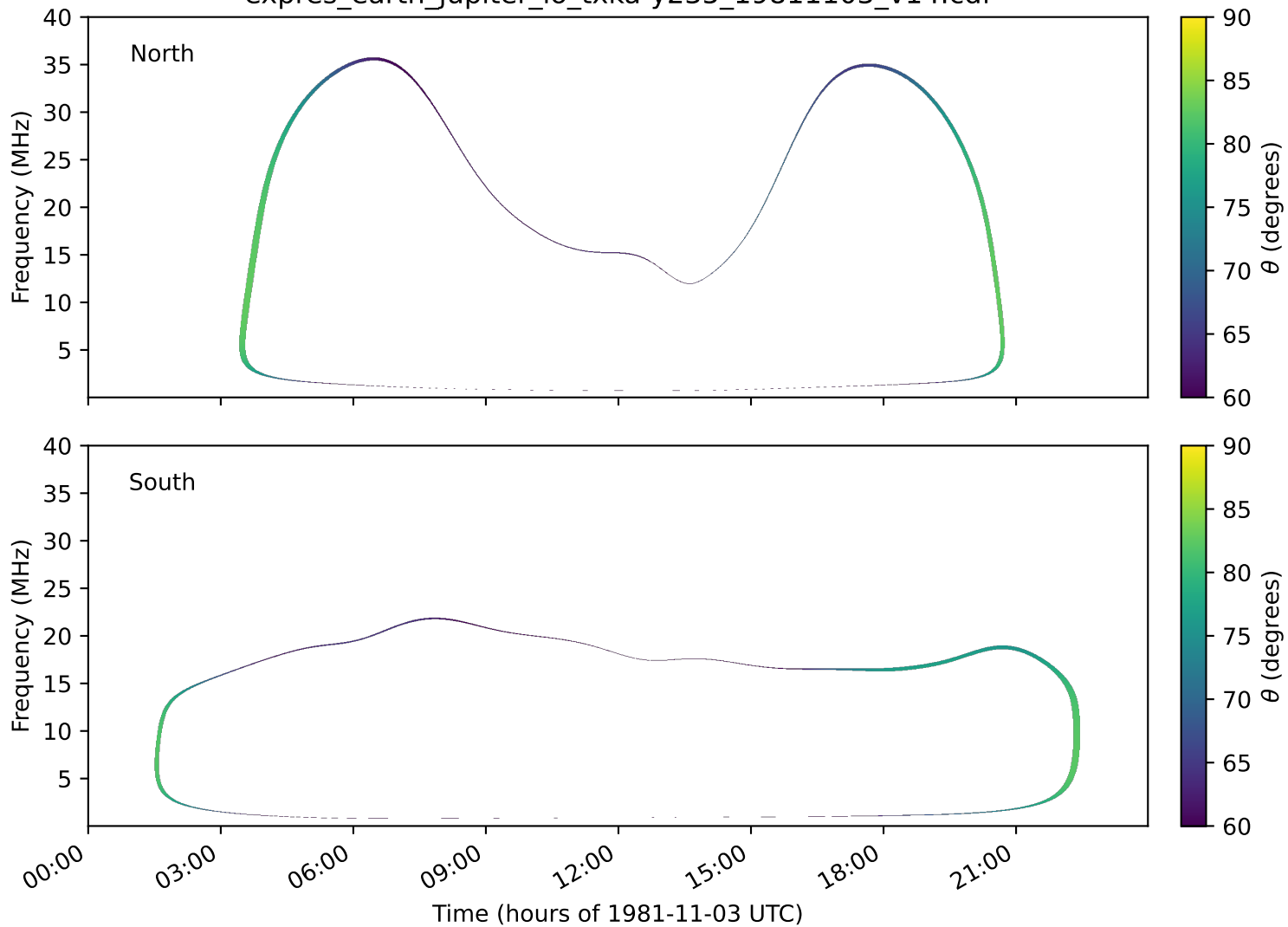
expres_earth_jupiter_io_txka-y235_19811103_v14.cdf
