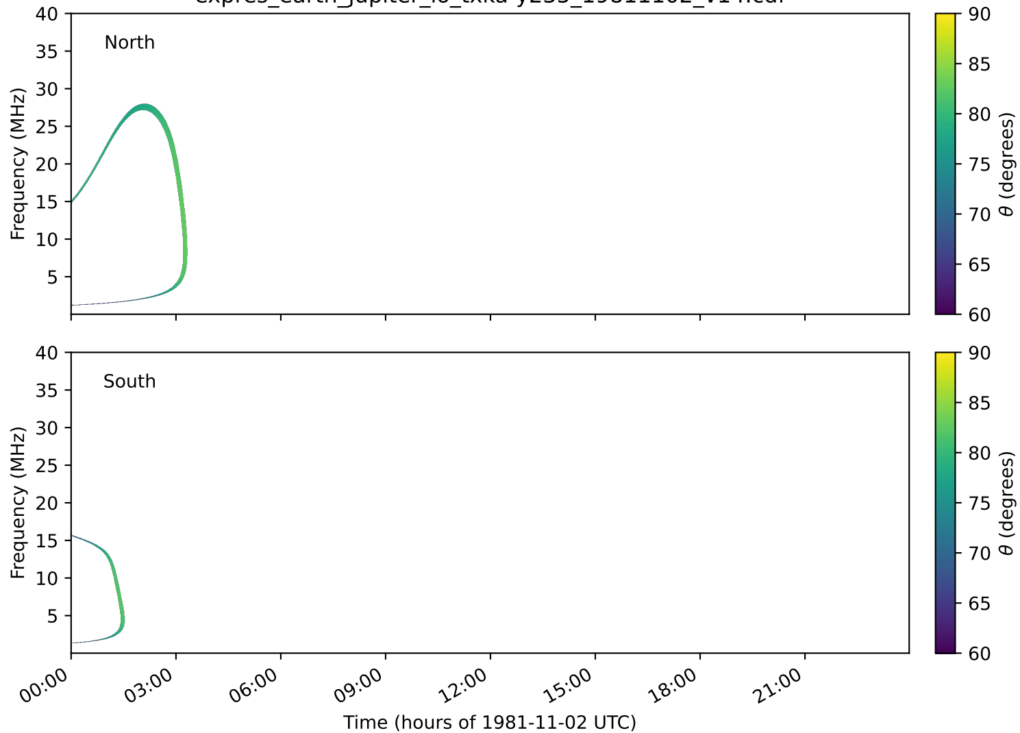
expres_earth_jupiter_io_txka-y235_19811102_v14.cdf
